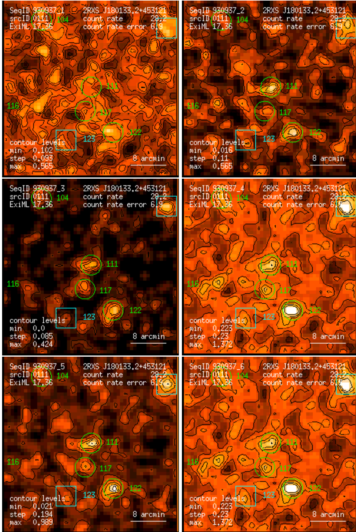
Figure 111: RASS 930937: detection 0111: band rate images, Gaussian filter: (1) PSPC channels 11 – 41, (2) 52 – 90, (3) 91 – 201, (4) 11 – 235, (5) 52 – 201, (6) 11 – 201. Broad band rates in counts/ks. Band rate contour levels in counts/ks/arcmin 2 .
