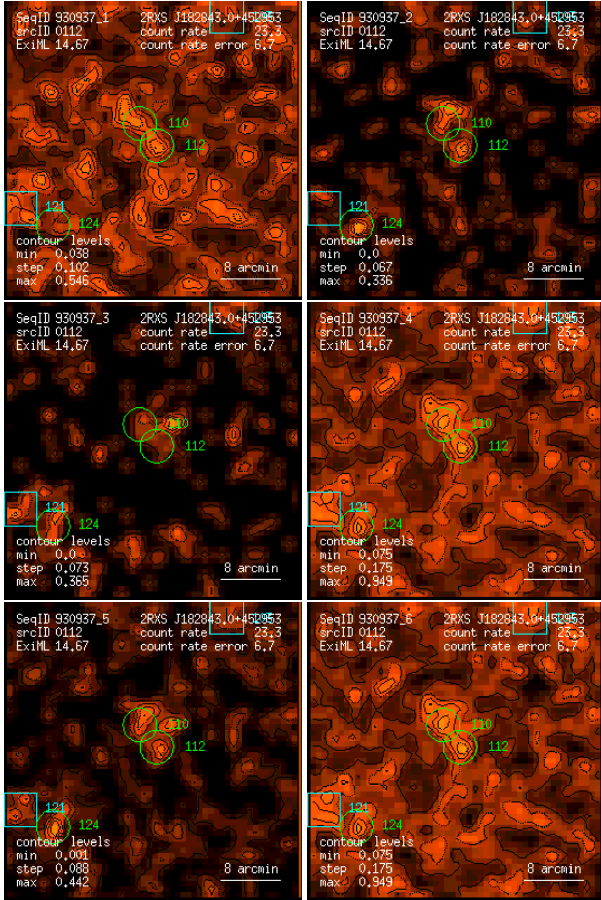
Figure 112: RASS 930937: detection 0112: band rate images, Gaussian filter: (1) PSPC channels 11 – 41, (2) 52 – 90, (3) 91 – 201, (4) 11 – 235, (5) 52 – 201, (6) 11 – 201. Broad band rates in counts/ks. Band rate contour levels in counts/ks/arcmin 2 .
