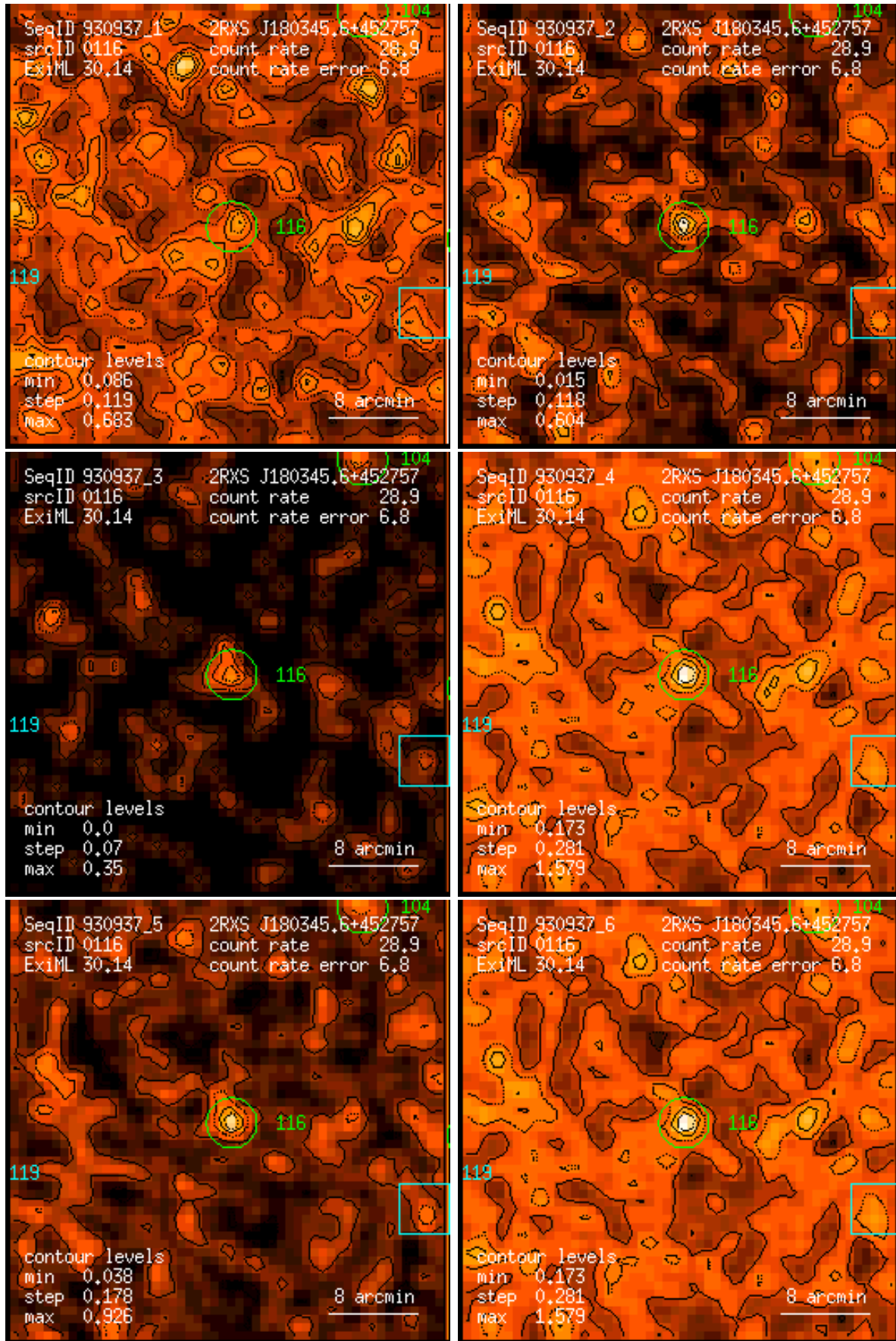
Figure 116: RASS 930937: detection 0116: band rate images, Gaussian filter: (1) PSPC channels 11 – 41, (2) 52 – 90, (3) 91 – 201, (4) 11 – 235, (5) 52 – 201, (6) 11 – 201. Broad band rates in counts/ks. Band rate contour levels in counts/ks/arcmin 2 .
