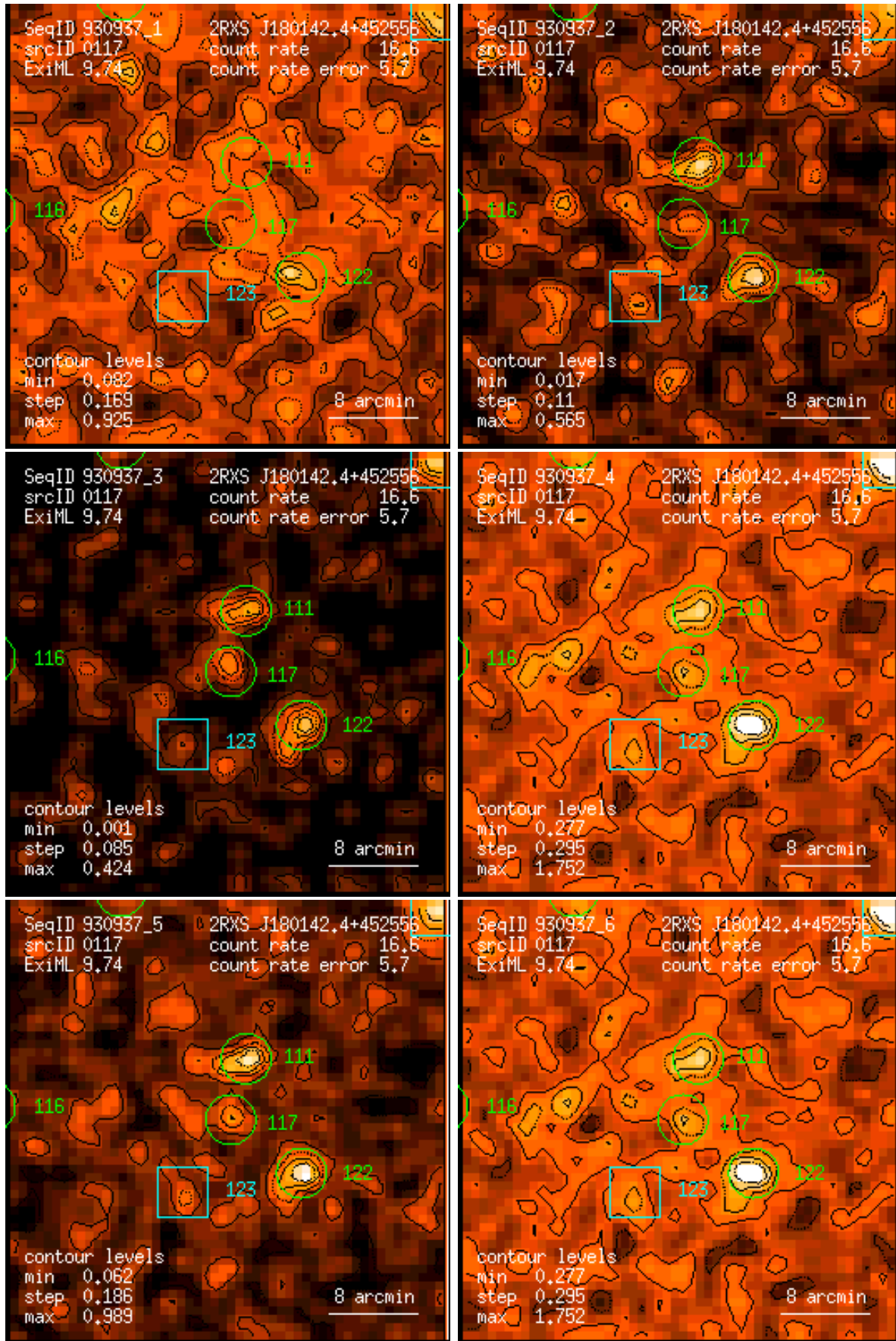
Figure 117: RASS 930937: detection 0117: band rate images, Gaussian filter: (1) PSPC channels 11 – 41, (2) 52 – 90, (3) 91 – 201, (4) 11 – 235, (5) 52 – 201, (6) 11 – 201. Broad band rates in counts/ks. Band rate contour levels in counts/ks/arcmin 2 .
