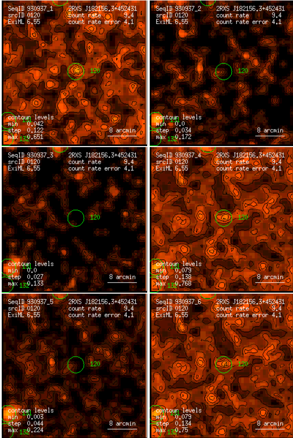
Figure 120: RASS 930937: detection 0120: band rate images, Gaussian filter: (1) PSPC channels 11 – 41, (2) 52 – 90, (3) 91 – 201, (4) 11 – 235, (5) 52 – 201, (6) 11 – 201. Broad band rates in counts/ks. Band rate contour levels in counts/ks/arcmin 2 .
