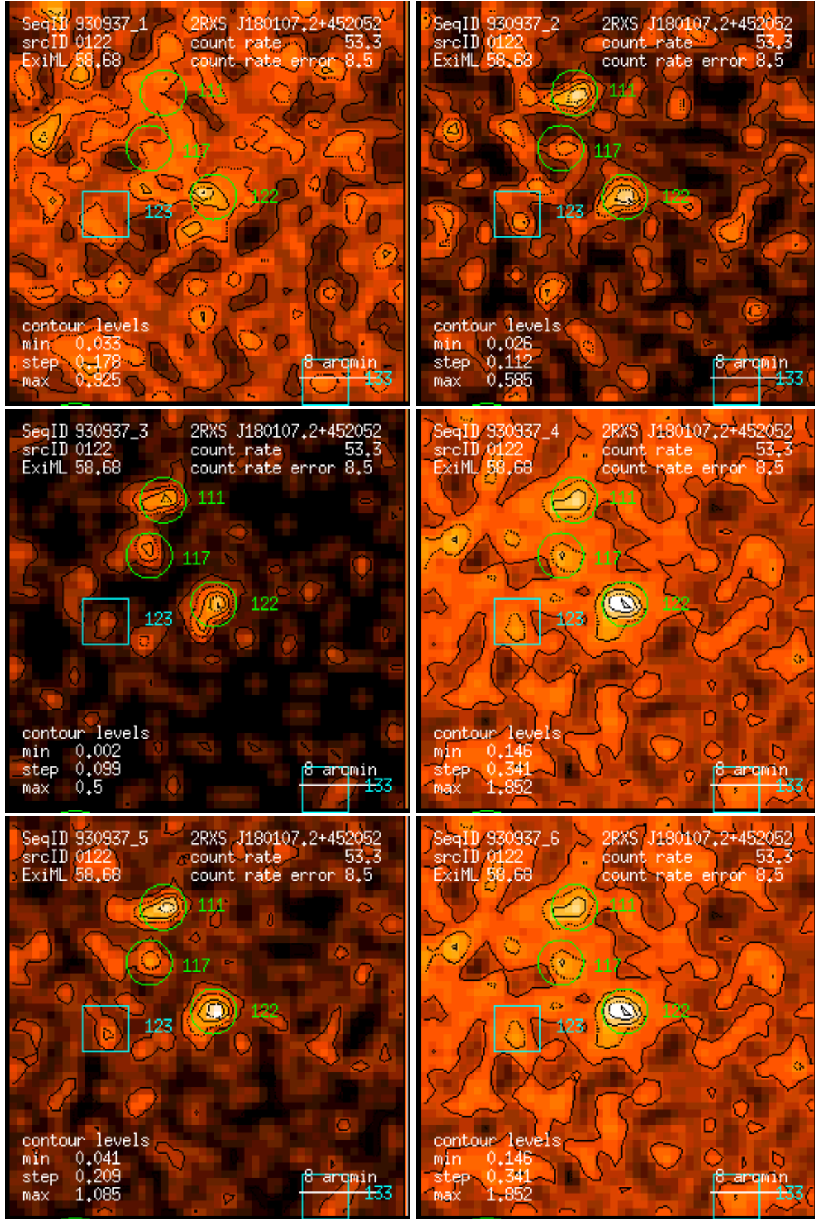
Figure 122: RASS 930937: detection 0122: band rate images, Gaussian filter: (1) PSPC channels 11 – 41, (2) 52 – 90, (3) 91 – 201, (4) 11 – 235, (5) 52 – 201, (6) 11 – 201. Broad band rates in counts/ks. Band rate contour levels in counts/ks/arcmin 2 .
