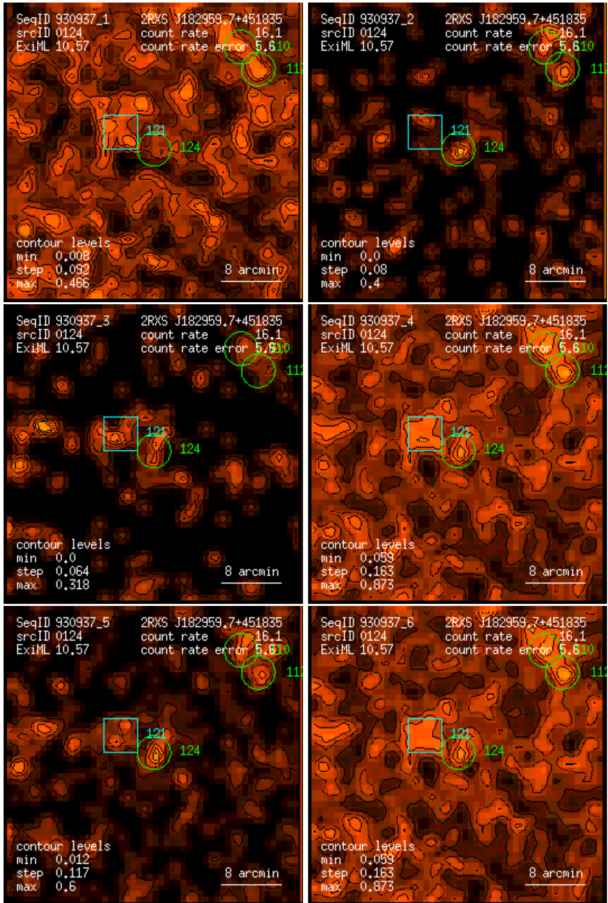
Figure 124: RASS 930937: detection 0124: band rate images, Gaussian filter: (1) PSPC channels 11 – 41, (2) 52 – 90, (3) 91 – 201, (4) 11 – 235, (5) 52 – 201, (6) 11 – 201. Broad band rates in counts/ks. Band rate contour levels in counts/ks/arcmin 2 .
