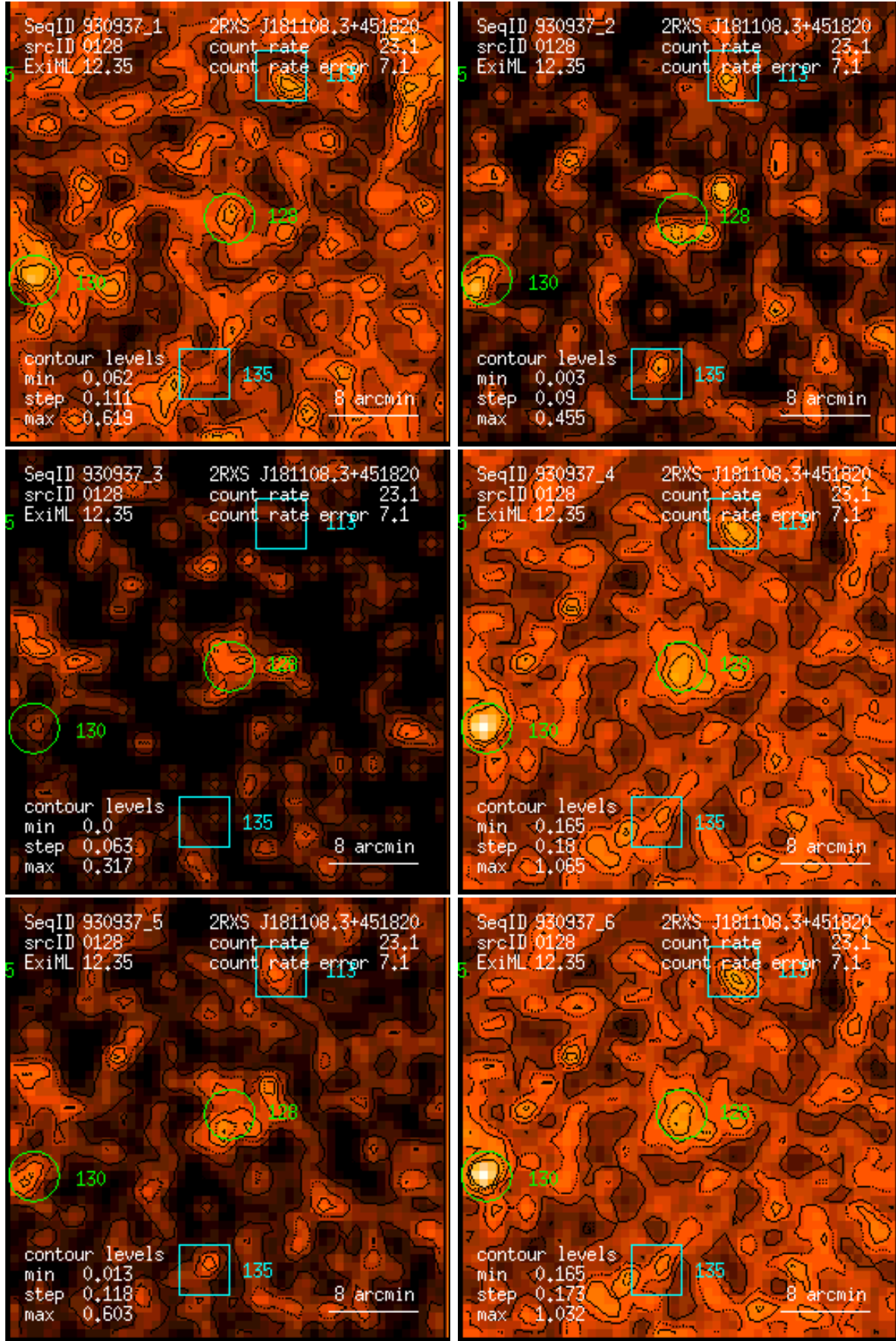
Figure 128: RASS 930937: detection 0128: band rate images, Gaussian filter: (1) PSPC channels 11 – 41, (2) 52 – 90, (3) 91 – 201, (4) 11 – 235, (5) 52 – 201, (6) 11 – 201. Broad band rates in counts/ks. Band rate contour levels in counts/ks/arcmin 2 .
