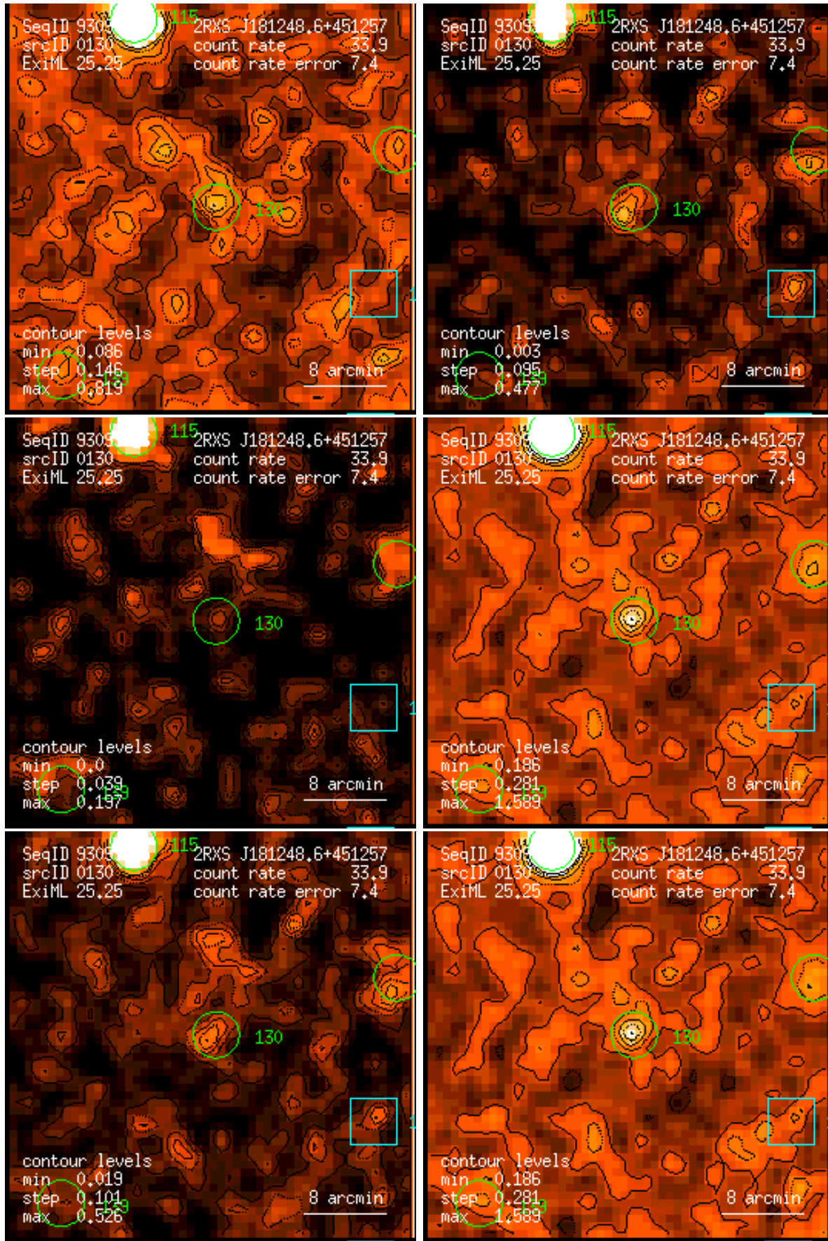
Figure 130: RASS 930937: detection 0130: band rate images, Gaussian filter: (1) PSPC channels 11 – 41, (2) 52 – 90, (3) 91 – 201, (4) 11 – 235, (5) 52 – 201, (6) 11 – 201. Broad band rates in counts/ks. Band rate contour levels in counts/ks/arcmin 2 .
