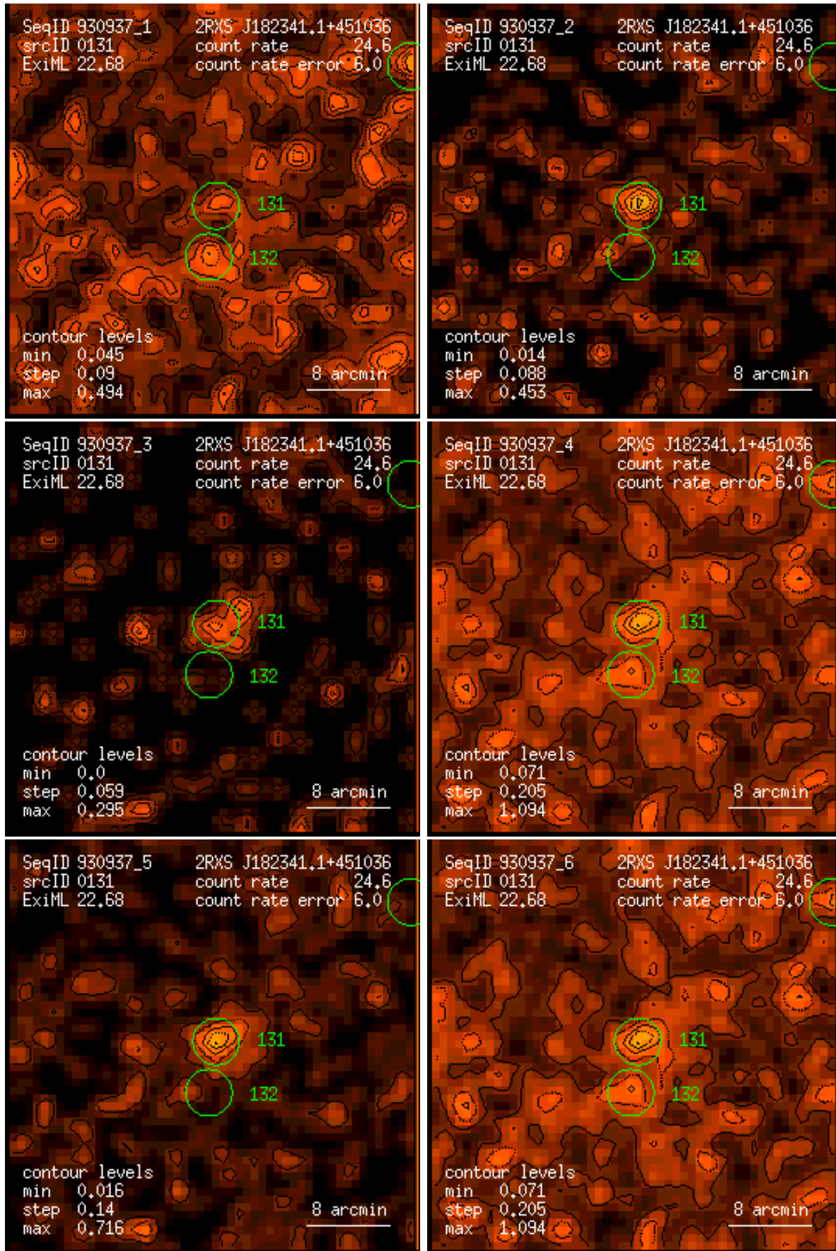
Figure 131: RASS 930937: detection 0131: band rate images, Gaussian filter: (1) PSPC channels 11 – 41, (2) 52 – 90, (3) 91 – 201, (4) 11 – 235, (5) 52 – 201, (6) 11 – 201. Broad band rates in counts/ks. Band rate contour levels in counts/ks/arcmin 2 .
