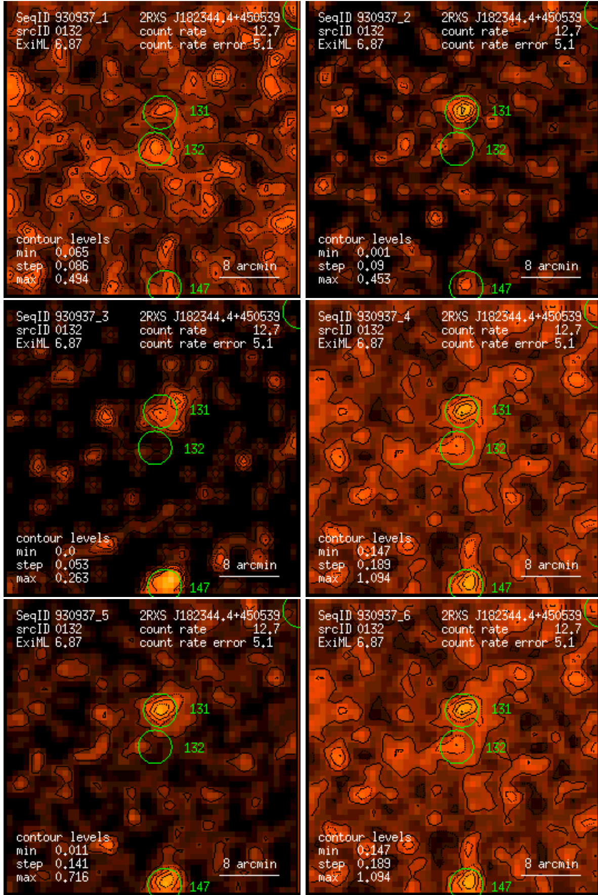
Figure 132: RASS 930937: detection 0132: band rate images, Gaussian filter: (1) PSPC channels 11 – 41, (2) 52 – 90, (3) 91 – 201, (4) 11 – 235, (5) 52 – 201, (6) 11 – 201. Broad band rates in counts/ks. Band rate contour levels in counts/ks/arcmin 2 .
