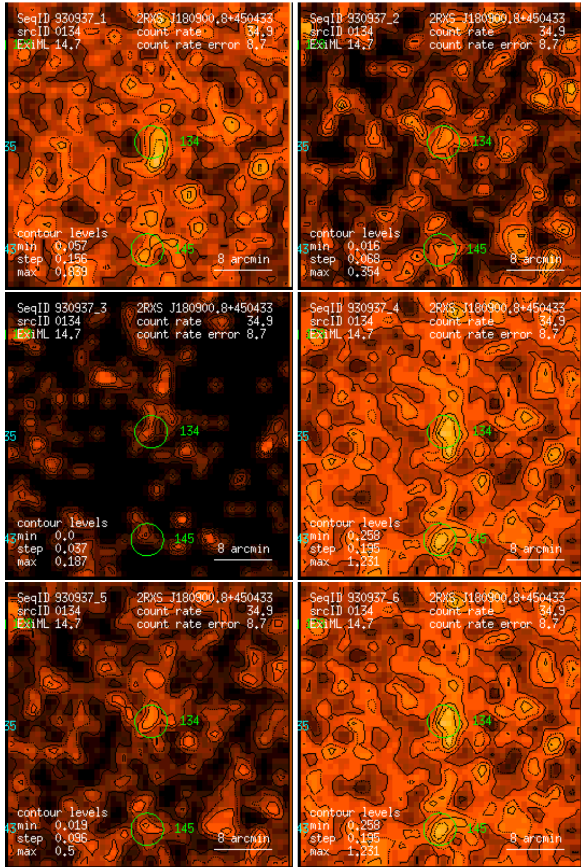
Figure 134: RASS 930937: detection 0134: band rate images, Gaussian filter: (1) PSPC channels 11 – 41, (2) 52 – 90, (3) 91 – 201, (4) 11 – 235, (5) 52 – 201, (6) 11 – 201. Broad band rates in counts/ks. Band rate contour levels in counts/ks/arcmin 2 .
