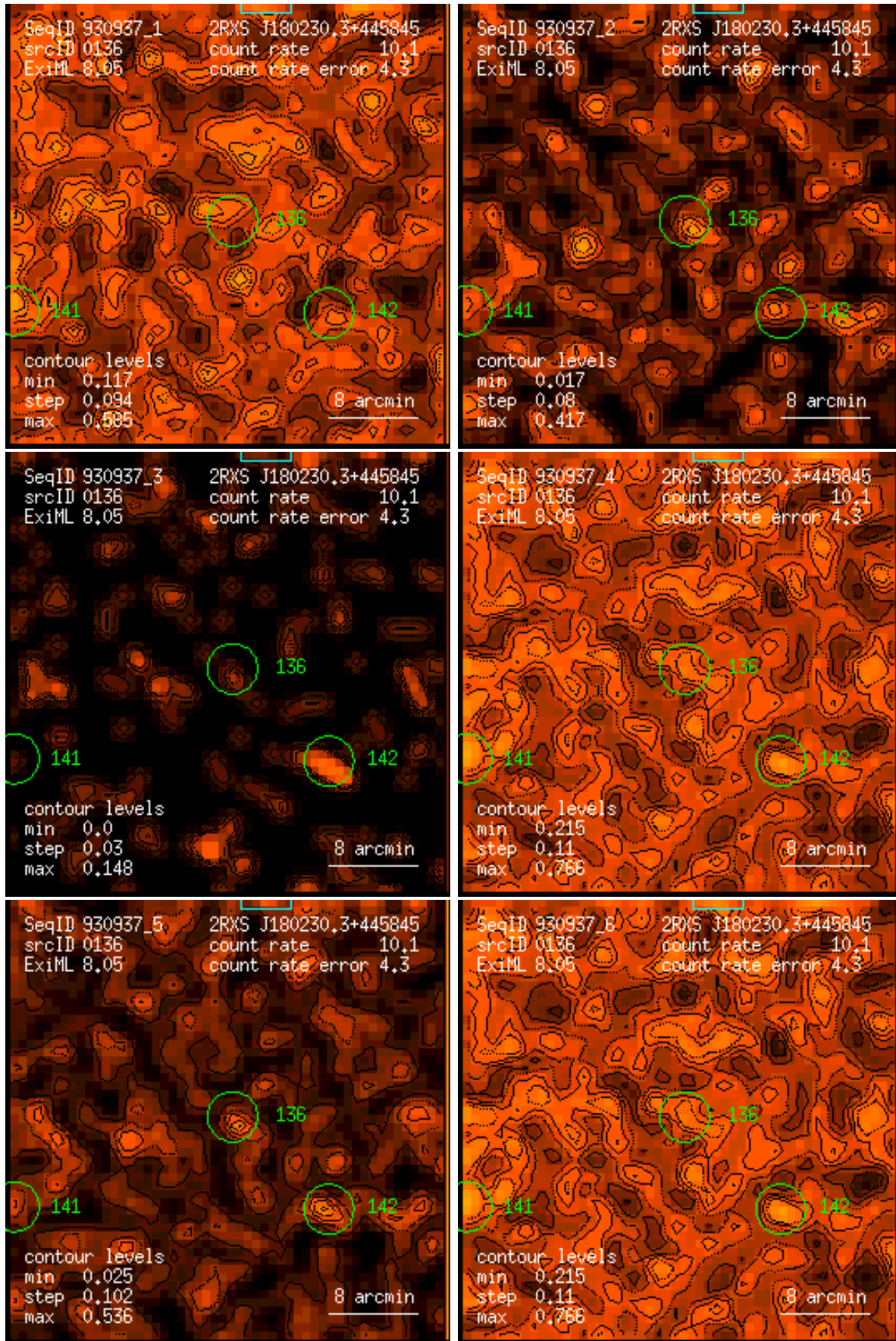
Figure 136: RASS 930937: detection 0136: band rate images, Gaussian filter: (1) PSPC channels 11 – 41, (2) 52 – 90, (3) 91 – 201, (4) 11 – 235, (5) 52 – 201, (6) 11 – 201. Broad band rates in counts/ks. Band rate contour levels in counts/ks/arcmin 2 .
