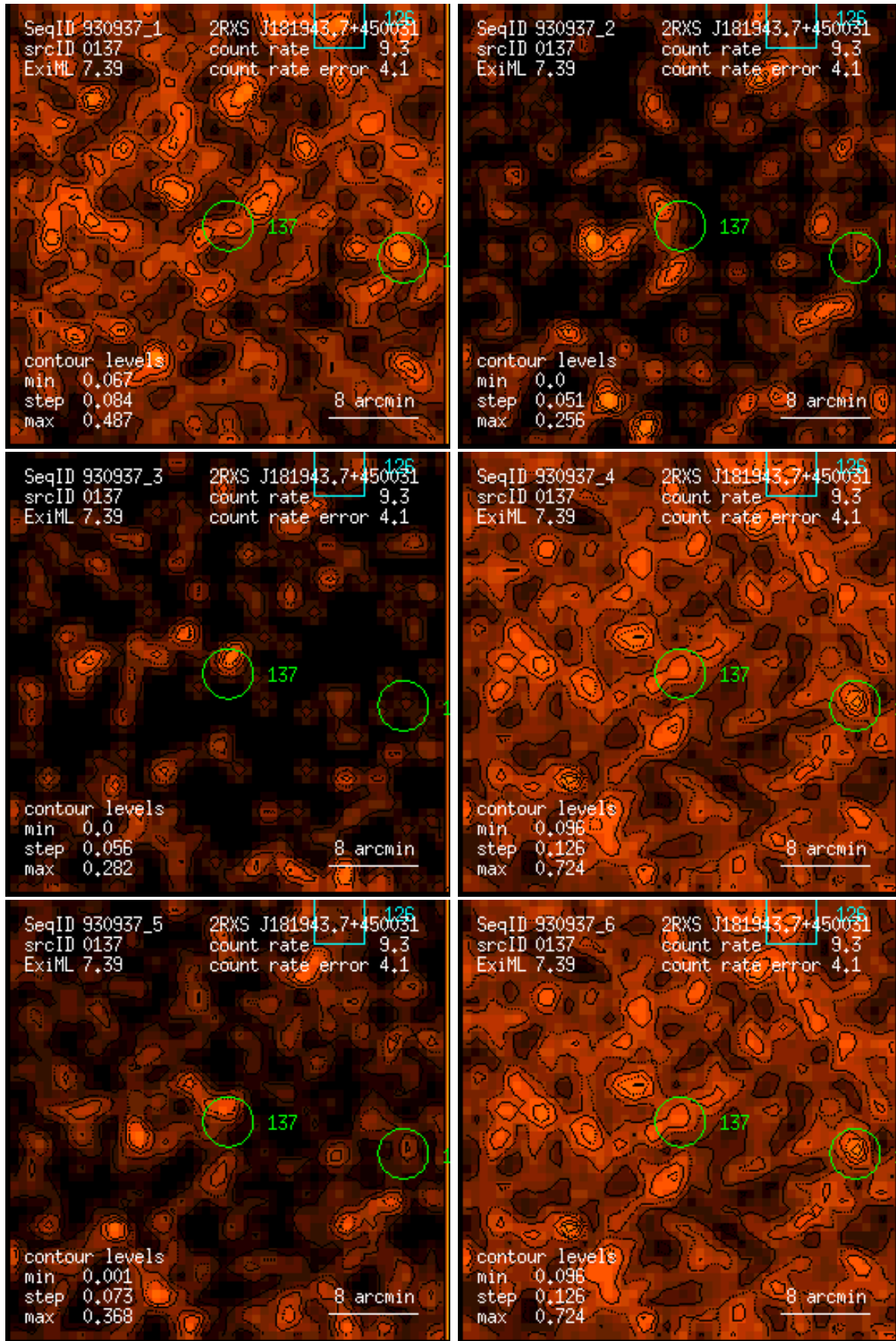
Figure 137: RASS 930937: detection 0137: band rate images, Gaussian filter: (1) PSPC channels 11 – 41, (2) 52 – 90, (3) 91 – 201, (4) 11 – 235, (5) 52 – 201, (6) 11 – 201. Broad band rates in counts/ks. Band rate contour levels in counts/ks/arcmin 2 .
