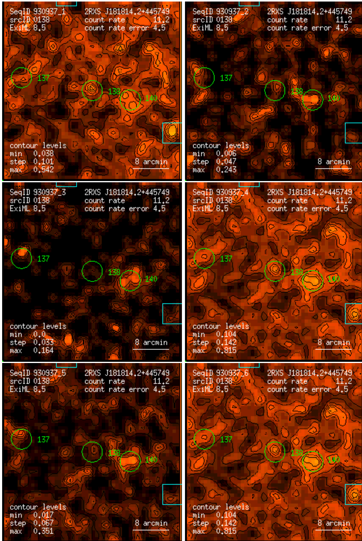
Figure 138: RASS 930937: detection 0138: band rate images, Gaussian filter: (1) PSPC channels 11 – 41, (2) 52 – 90, (3) 91 – 201, (4) 11 – 235, (5) 52 – 201, (6) 11 – 201. Broad band rates in counts/ks. Band rate contour levels in counts/ks/arcmin 2 .
