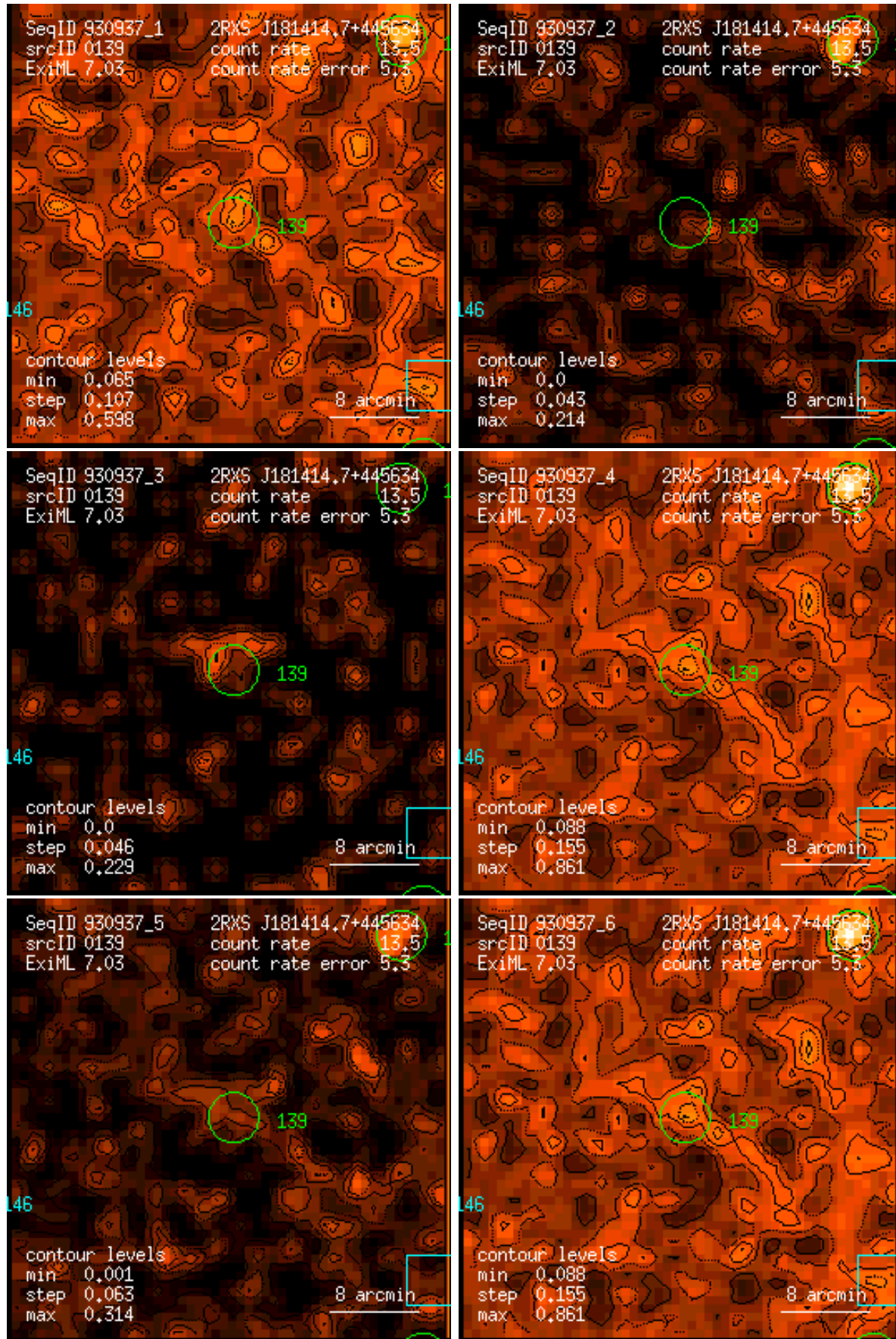
Figure 139: RASS 930937: detection 0139: band rate images, Gaussian filter: (1) PSPC channels 11 – 41, (2) 52 – 90, (3) 91 – 201, (4) 11 – 235, (5) 52 – 201, (6) 11 – 201. Broad band rates in counts/ks. Band rate contour levels in counts/ks/arcmin 2 .
