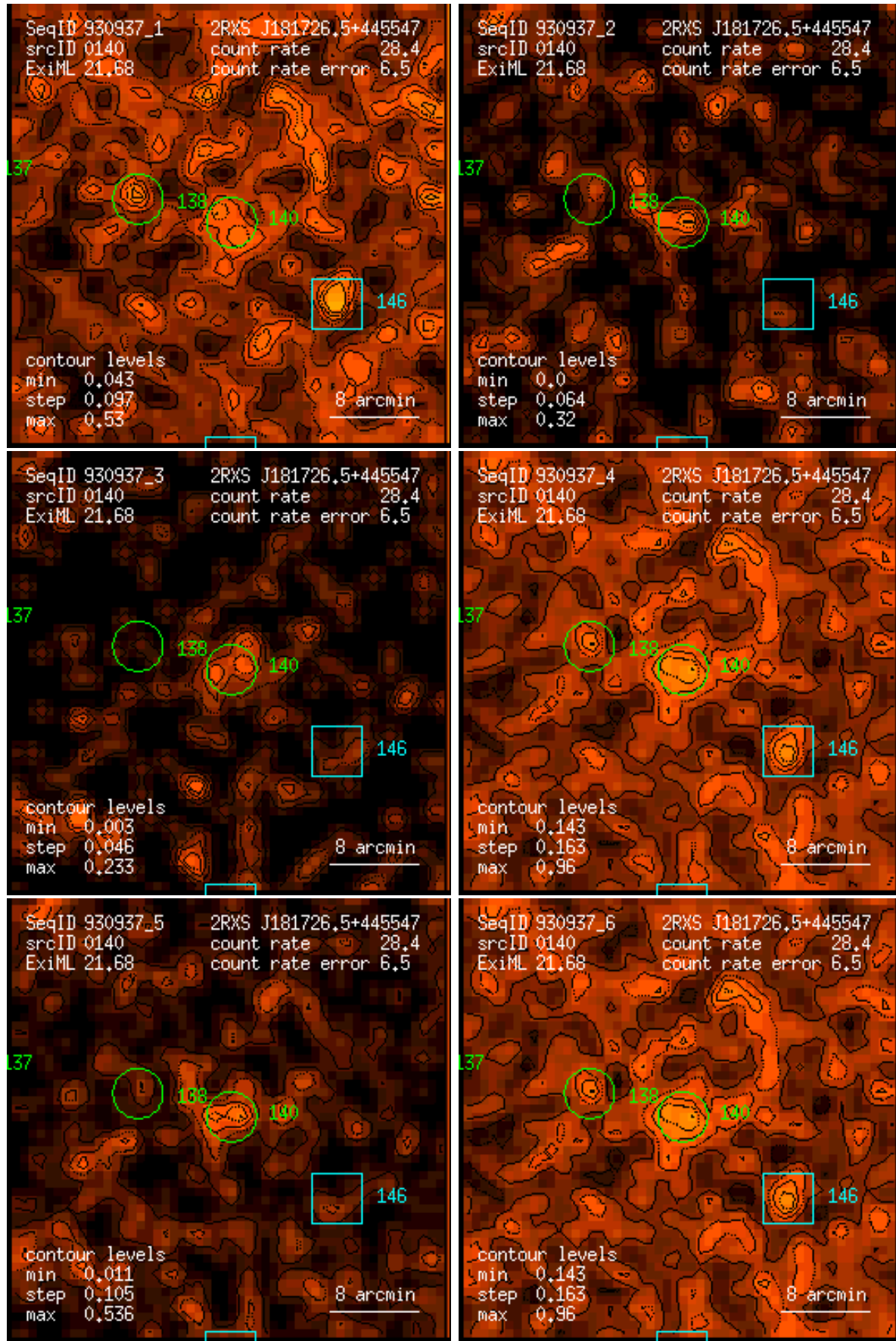
Figure 140: RASS 930937: detection 0140: band rate images, Gaussian filter: (1) PSPC channels 11 – 41, (2) 52 – 90, (3) 91 – 201, (4) 11 – 235, (5) 52 – 201, (6) 11 – 201. Broad band rates in counts/ks. Band rate contour levels in counts/ks/arcmin 2 .
