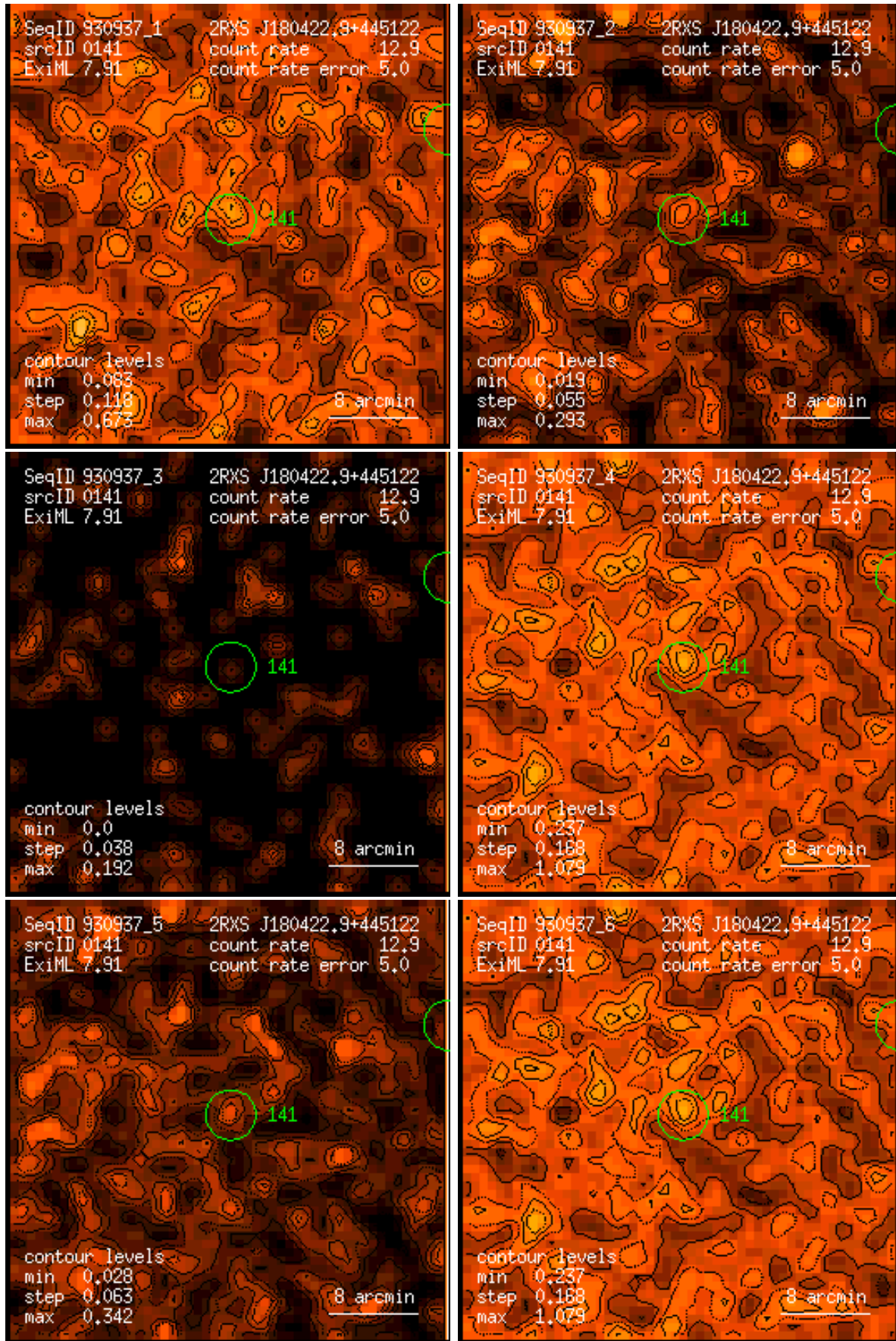
Figure 141: RASS 930937: detection 0141: band rate images, Gaussian filter: (1) PSPC channels 11 – 41, (2) 52 – 90, (3) 91 – 201, (4) 11 – 235, (5) 52 – 201, (6) 11 – 201. Broad band rates in counts/ks. Band rate contour levels in counts/ks/arcmin 2 .
