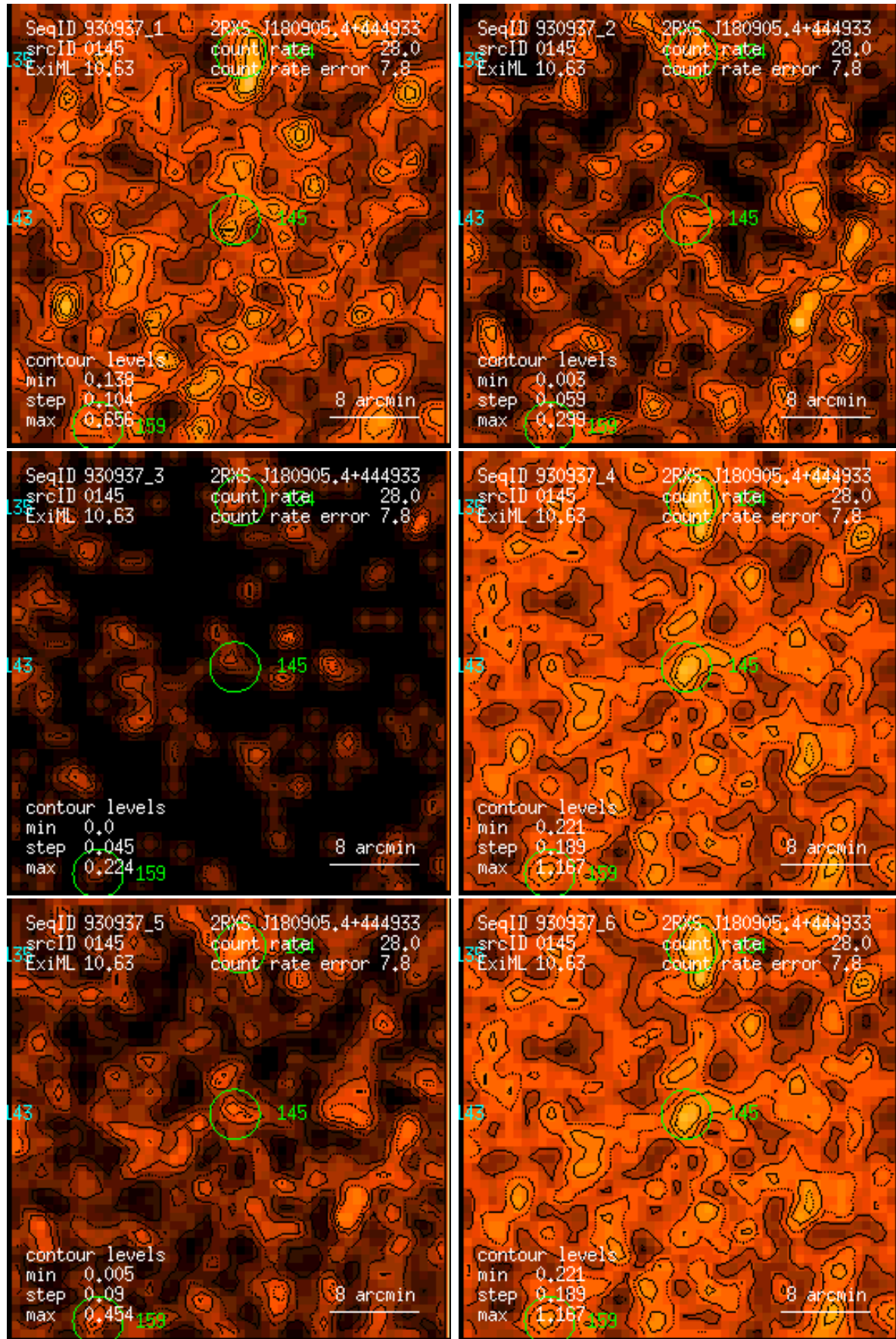
Figure 145: RASS 930937: detection 0145: band rate images, Gaussian filter: (1) PSPC channels 11 – 41, (2) 52 – 90, (3) 91 – 201, (4) 11 – 235, (5) 52 – 201, (6) 11 – 201. Broad band rates in counts/ks. Band rate contour levels in counts/ks/arcmin 2 .
