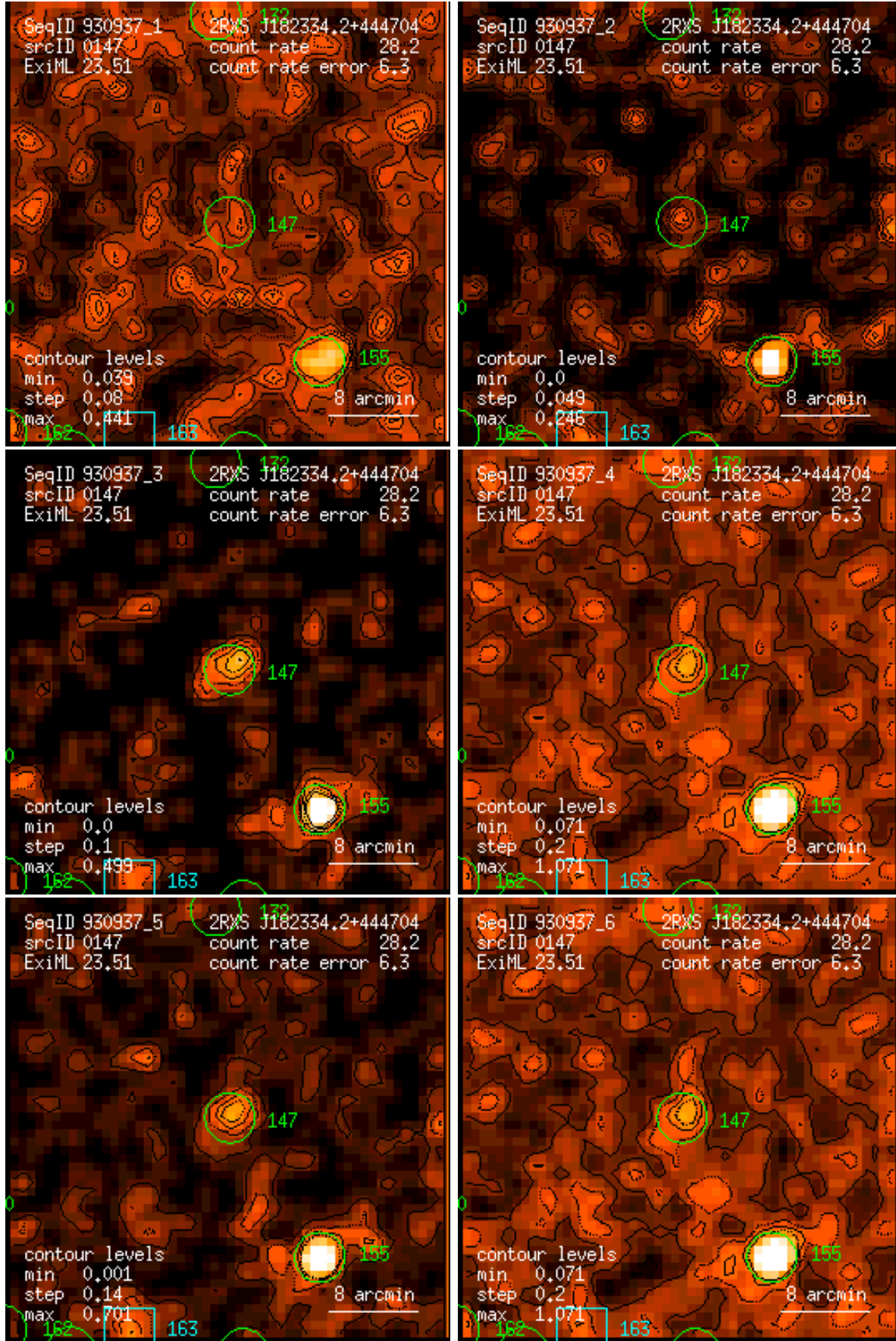
Figure 147: RASS 930937: detection 0147: band rate images, Gaussian filter: (1) PSPC channels 11 – 41, (2) 52 – 90, (3) 91 – 201, (4) 11 – 235, (5) 52 – 201, (6) 11 – 201. Broad band rates in counts/ks. Band rate contour levels in counts/ks/arcmin 2 .
