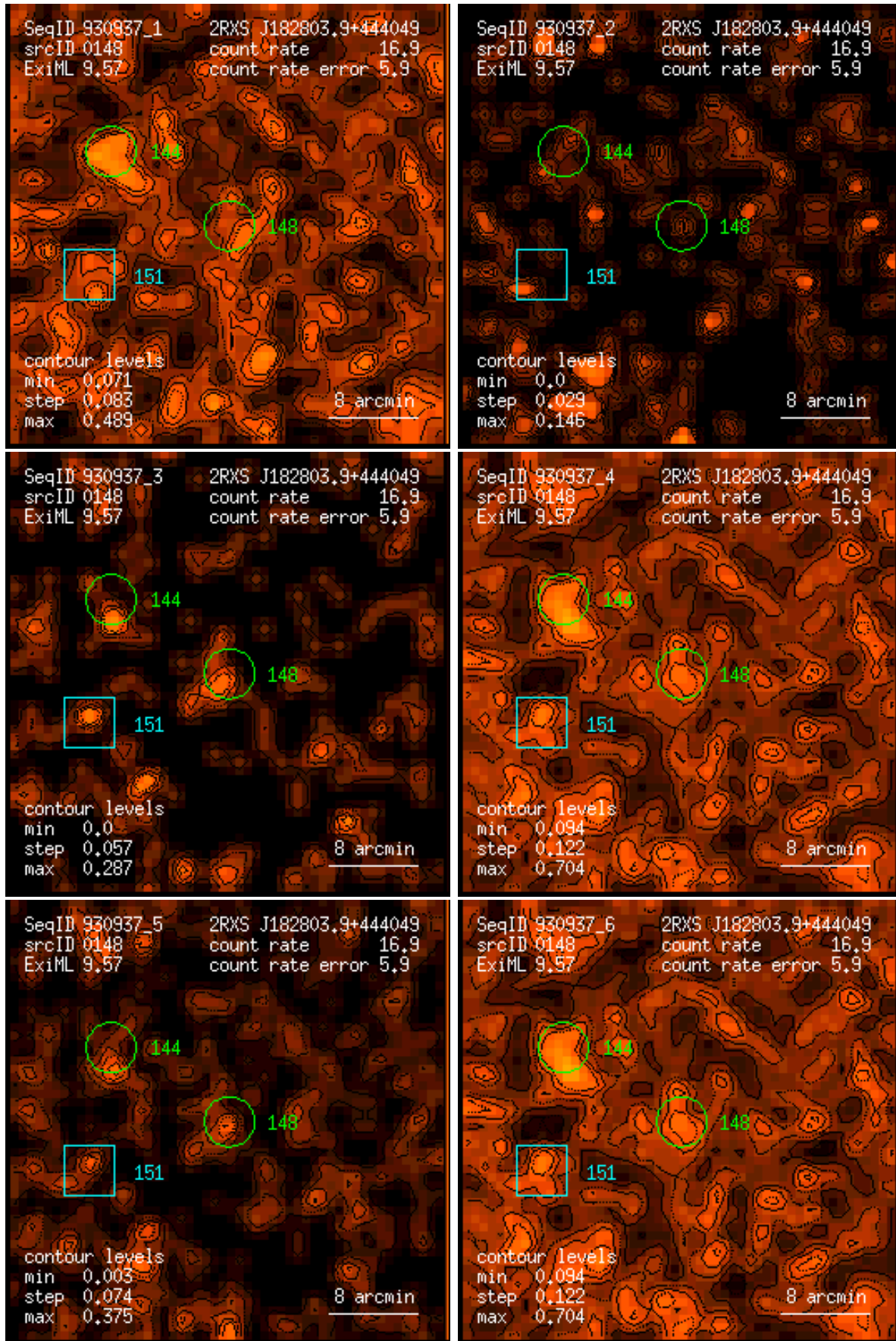
Figure 148: RASS 930937: detection 0148: band rate images, Gaussian filter: (1) PSPC channels 11 – 41, (2) 52 – 90, (3) 91 – 201, (4) 11 – 235, (5) 52 – 201, (6) 11 – 201. Broad band rates in counts/ks. Band rate contour levels in counts/ks/arcmin 2 .
