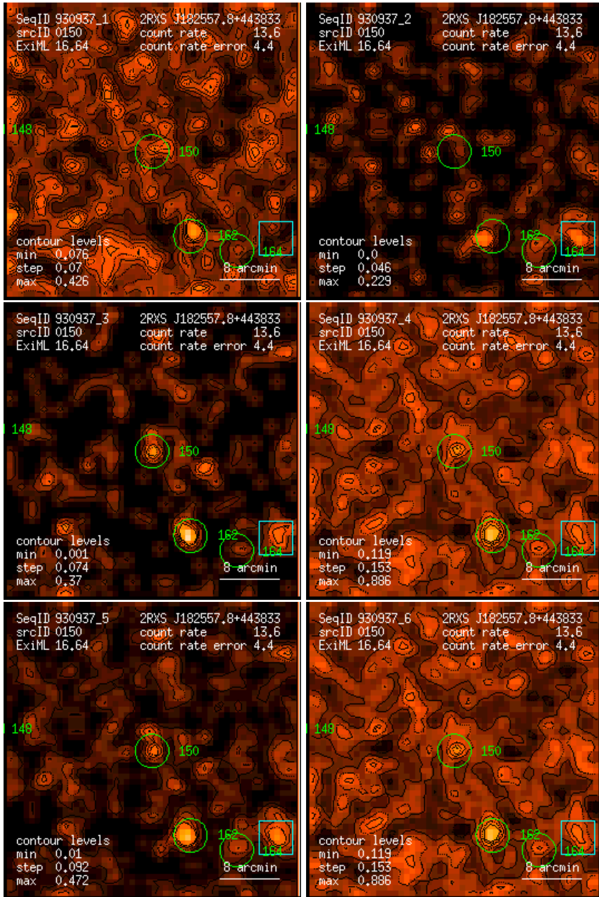
Figure 150: RASS 930937: detection 0150: band rate images, Gaussian filter: (1) PSPC channels 11 – 41, (2) 52 – 90, (3) 91 – 201, (4) 11 – 235, (5) 52 – 201, (6) 11 – 201. Broad band rates in counts/ks. Band rate contour levels in counts/ks/arcmin 2 .
