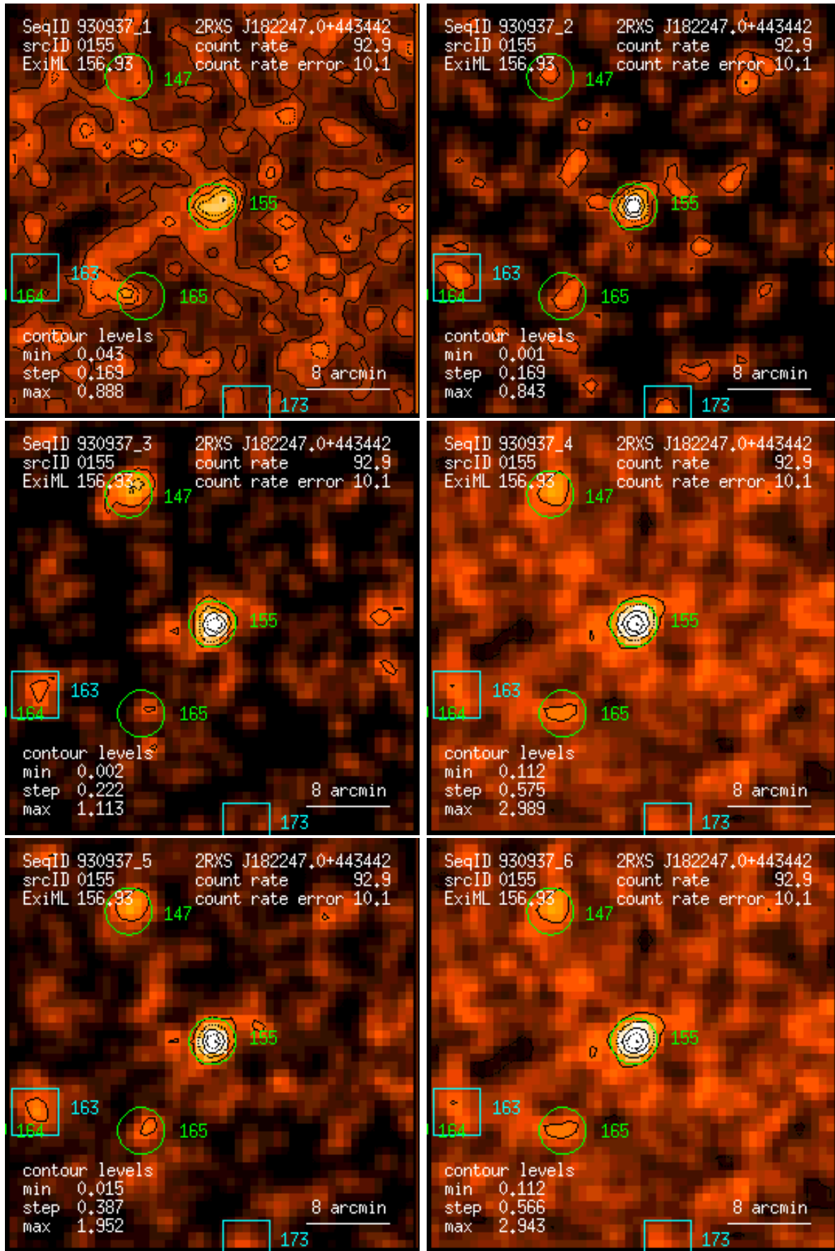
Figure 155: RASS 930937: detection 0155: band rate images, Gaussian filter: (1) PSPC channels 11 – 41, (2) 52 – 90, (3) 91 – 201, (4) 11 – 235, (5) 52 – 201, (6) 11 – 201. Broad band rates in counts/ks. Band rate contour levels in counts/ks/arcmin 2 .
