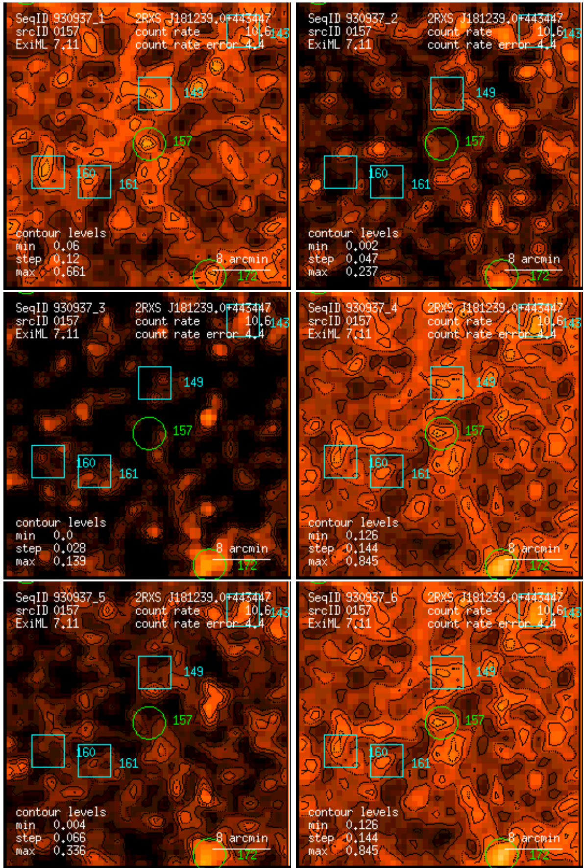
Figure 157: RASS 930937: detection 0157: band rate images, Gaussian filter: (1) PSPC channels 11 – 41, (2) 52 – 90, (3) 91 – 201, (4) 11 – 235, (5) 52 – 201, (6) 11 – 201. Broad band rates in counts/ks. Band rate contour levels in counts/ks/arcmin 2 .
