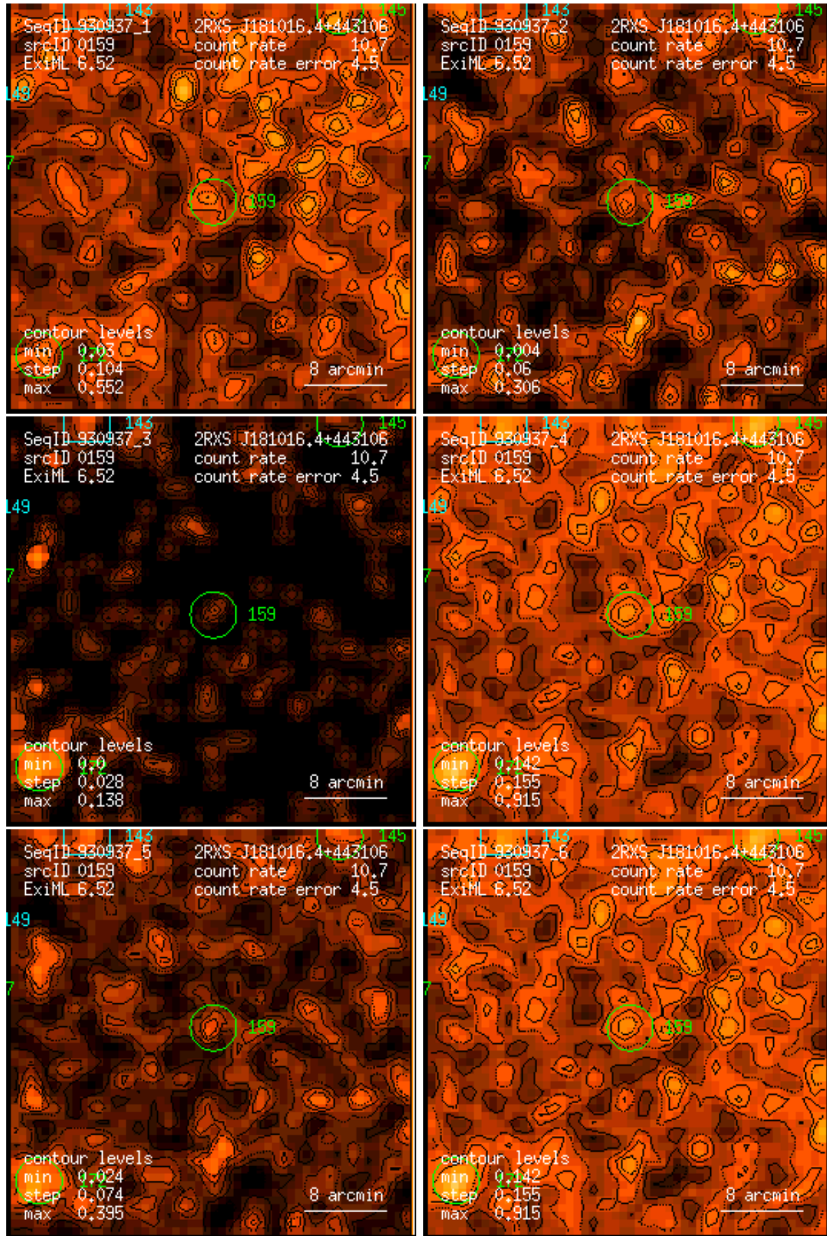
Figure 159: RASS 930937: detection 0159: band rate images, Gaussian filter: (1) PSPC channels 11 – 41, (2) 52 – 90, (3) 91 – 201, (4) 11 – 235, (5) 52 – 201, (6) 11 – 201. Broad band rates in counts/ks. Band rate contour levels in counts/ks/arcmin 2 .
