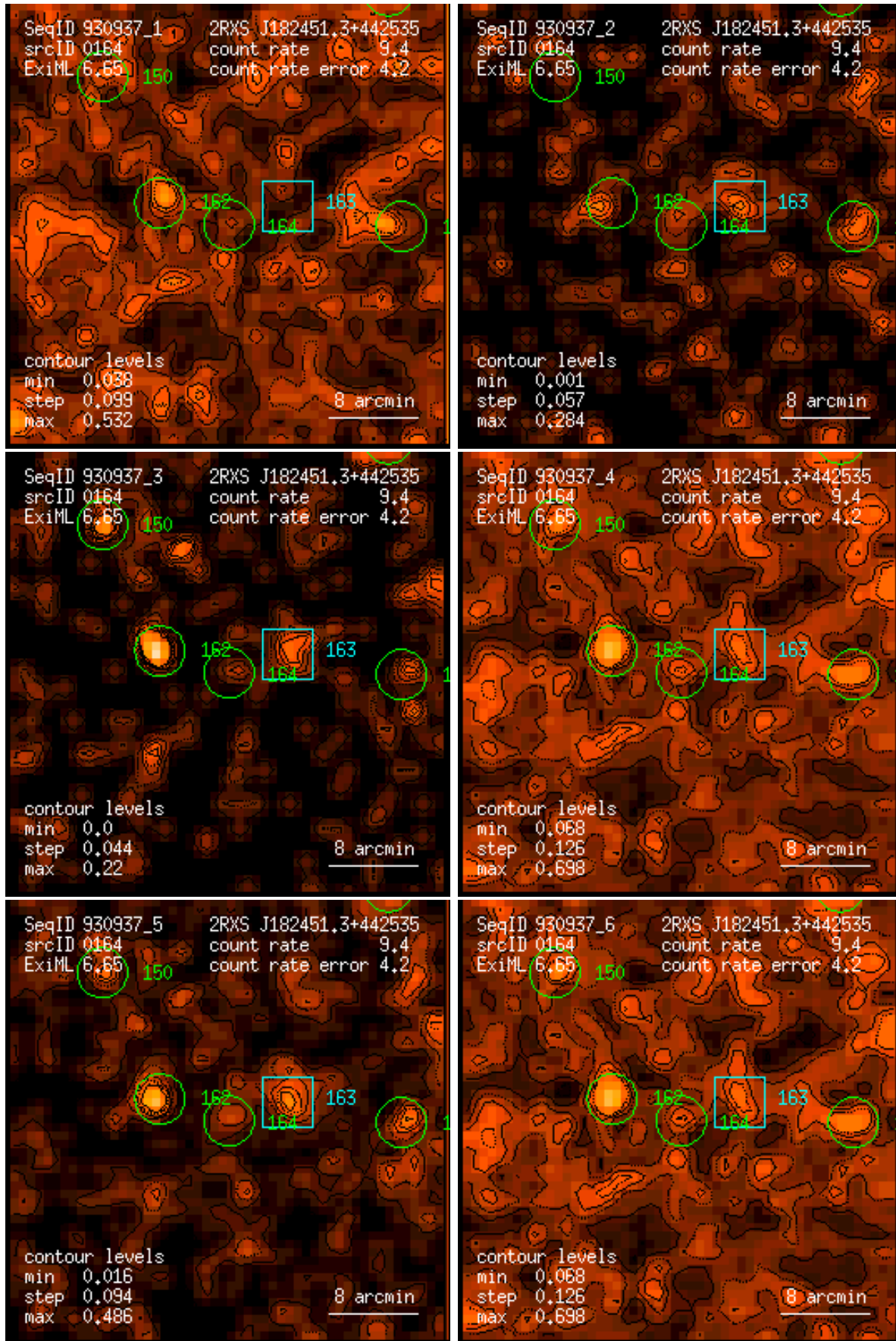
Figure 164: RASS 930937: detection 0164: band rate images, Gaussian filter: (1) PSPC channels 11 – 41, (2) 52 – 90, (3) 91 – 201, (4) 11 – 235, (5) 52 – 201, (6) 11 – 201. Broad band rates in counts/ks. Band rate contour levels in counts/ks/arcmin 2 .
