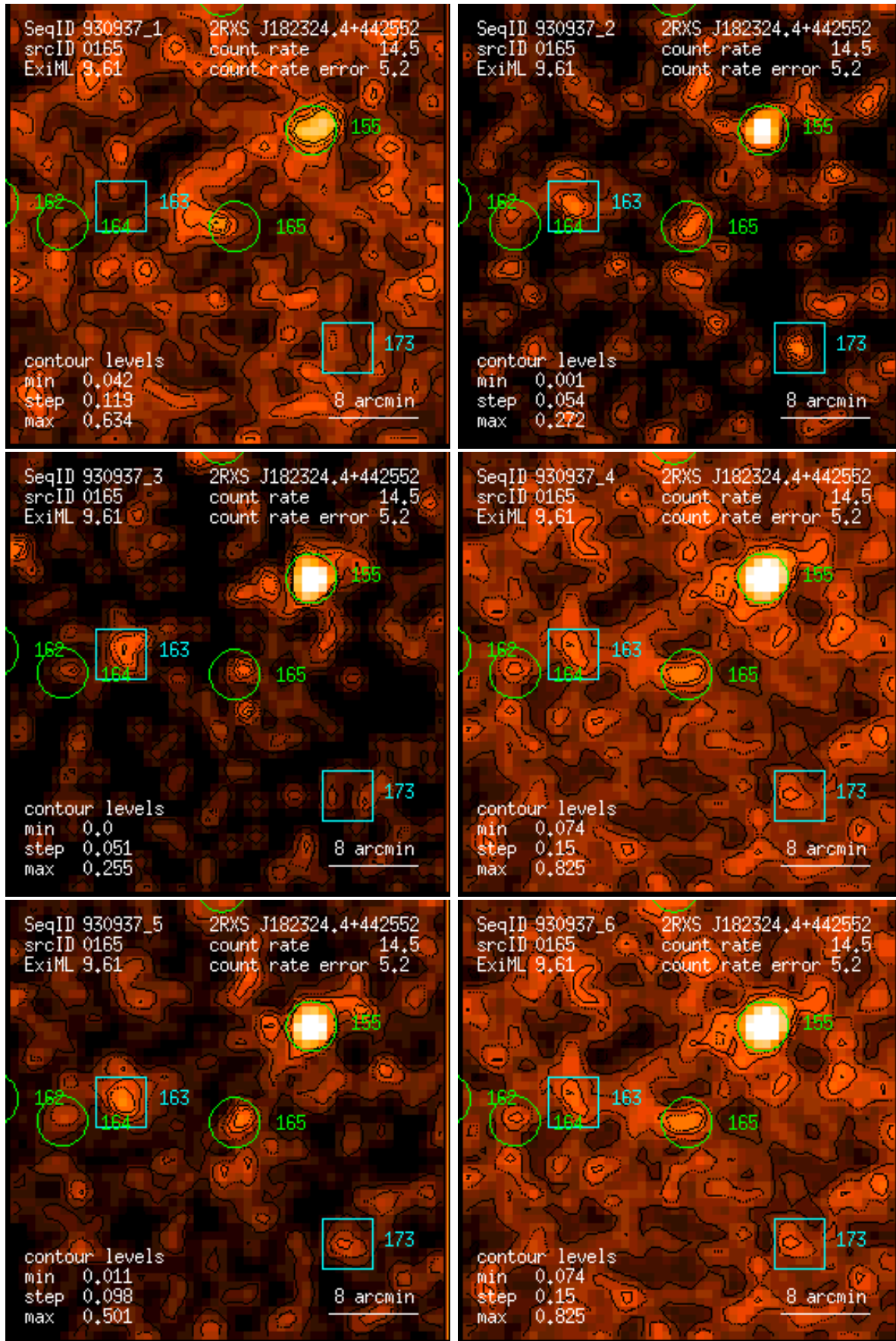
Figure 165: RASS 930937: detection 0165: band rate images, Gaussian filter: (1) PSPC channels 11 – 41, (2) 52 – 90, (3) 91 – 201, (4) 11 – 235, (5) 52 – 201, (6) 11 – 201. Broad band rates in counts/ks. Band rate contour levels in counts/ks/arcmin 2 .
