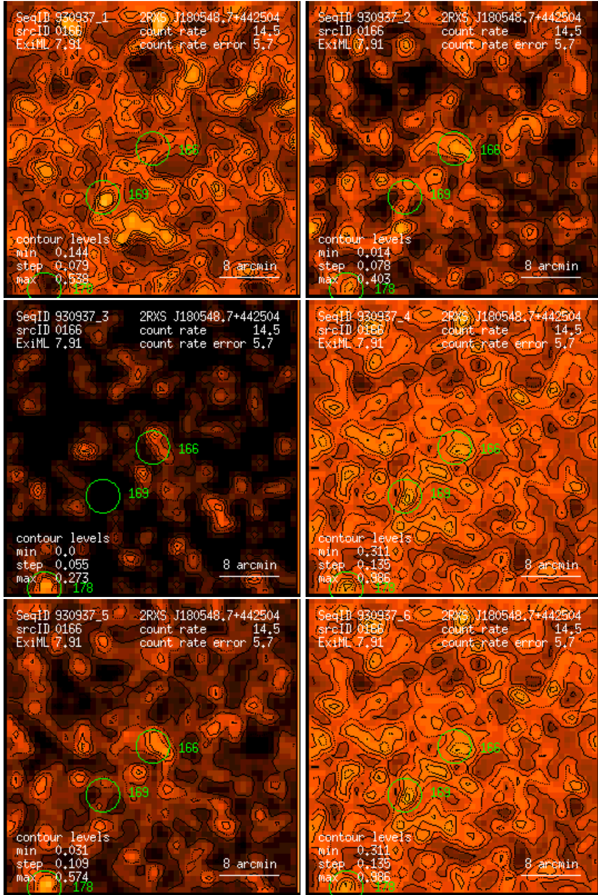
Figure 166: RASS 930937: detection 0166: band rate images, Gaussian filter: (1) PSPC channels 11 – 41, (2) 52 – 90, (3) 91 – 201, (4) 11 – 235, (5) 52 – 201, (6) 11 – 201. Broad band rates in counts/ks. Band rate contour levels in counts/ks/arcmin 2 .
