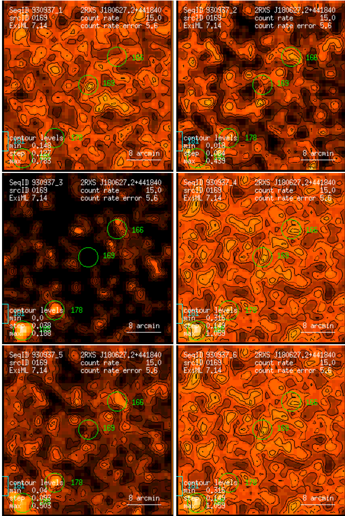
Figure 169: RASS 930937: detection 0169: band rate images, Gaussian filter: (1) PSPC channels 11 – 41, (2) 52 – 90, (3) 91 – 201, (4) 11 – 235, (5) 52 – 201, (6) 11 – 201. Broad band rates in counts/ks. Band rate contour levels in counts/ks/arcmin 2 .
