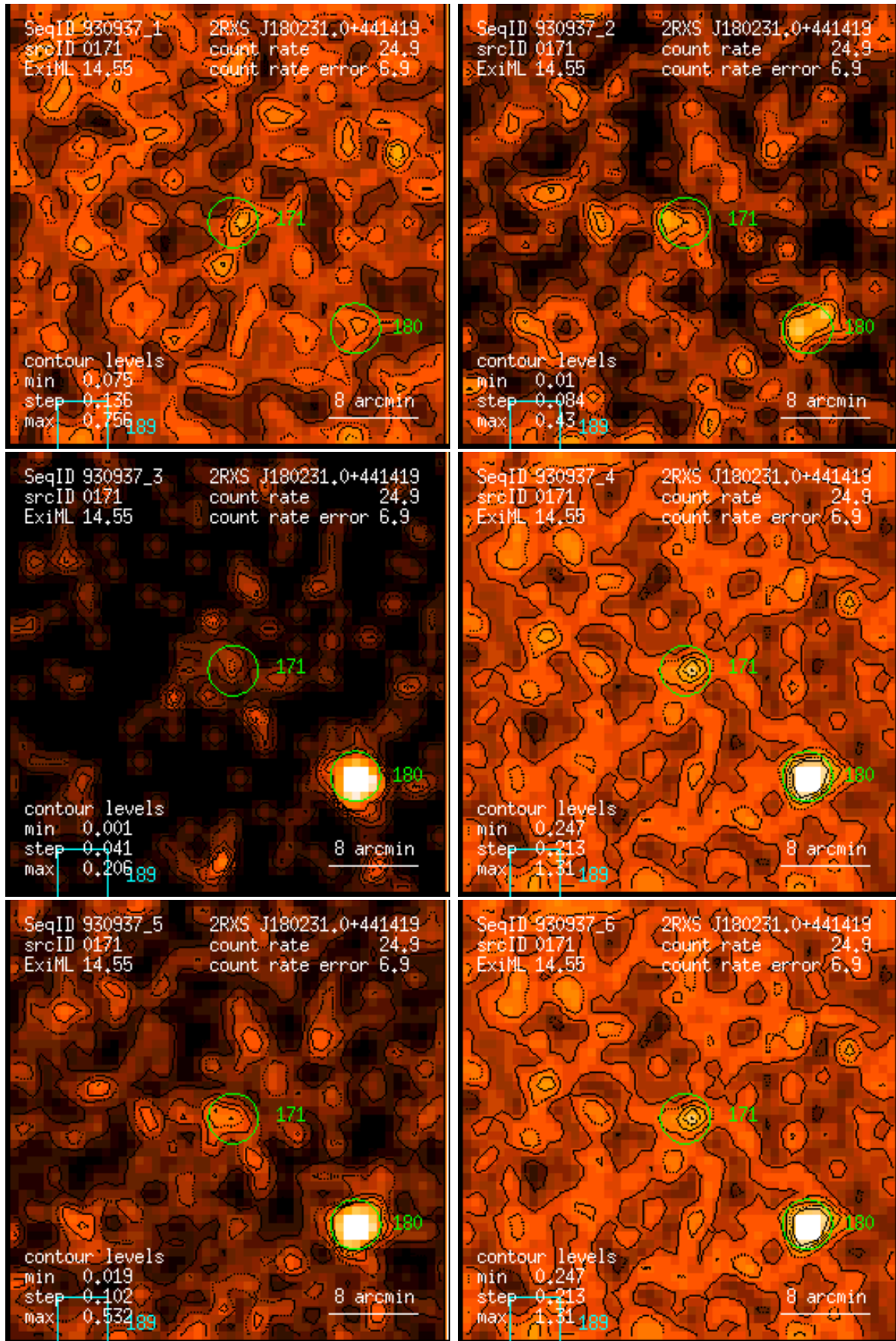
Figure 171: RASS 930937: detection 0171: band rate images, Gaussian filter: (1) PSPC channels 11 – 41, (2) 52 – 90, (3) 91 – 201, (4) 11 – 235, (5) 52 – 201, (6) 11 – 201. Broad band rates in counts/ks. Band rate contour levels in counts/ks/arcmin 2 .
