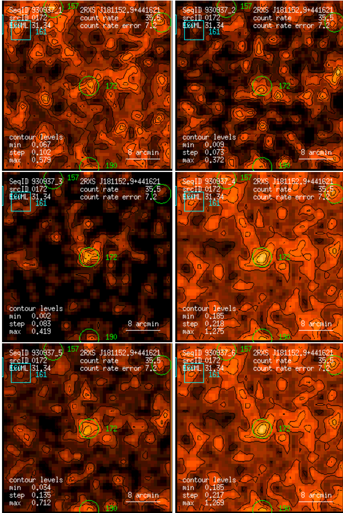
Figure 172: RASS 930937: detection 0172: band rate images, Gaussian filter: (1) PSPC channels 11 – 41, (2) 52 – 90, (3) 91 – 201, (4) 11 – 235, (5) 52 – 201, (6) 11 – 201. Broad band rates in counts/ks. Band rate contour levels in counts/ks/arcmin 2 .
