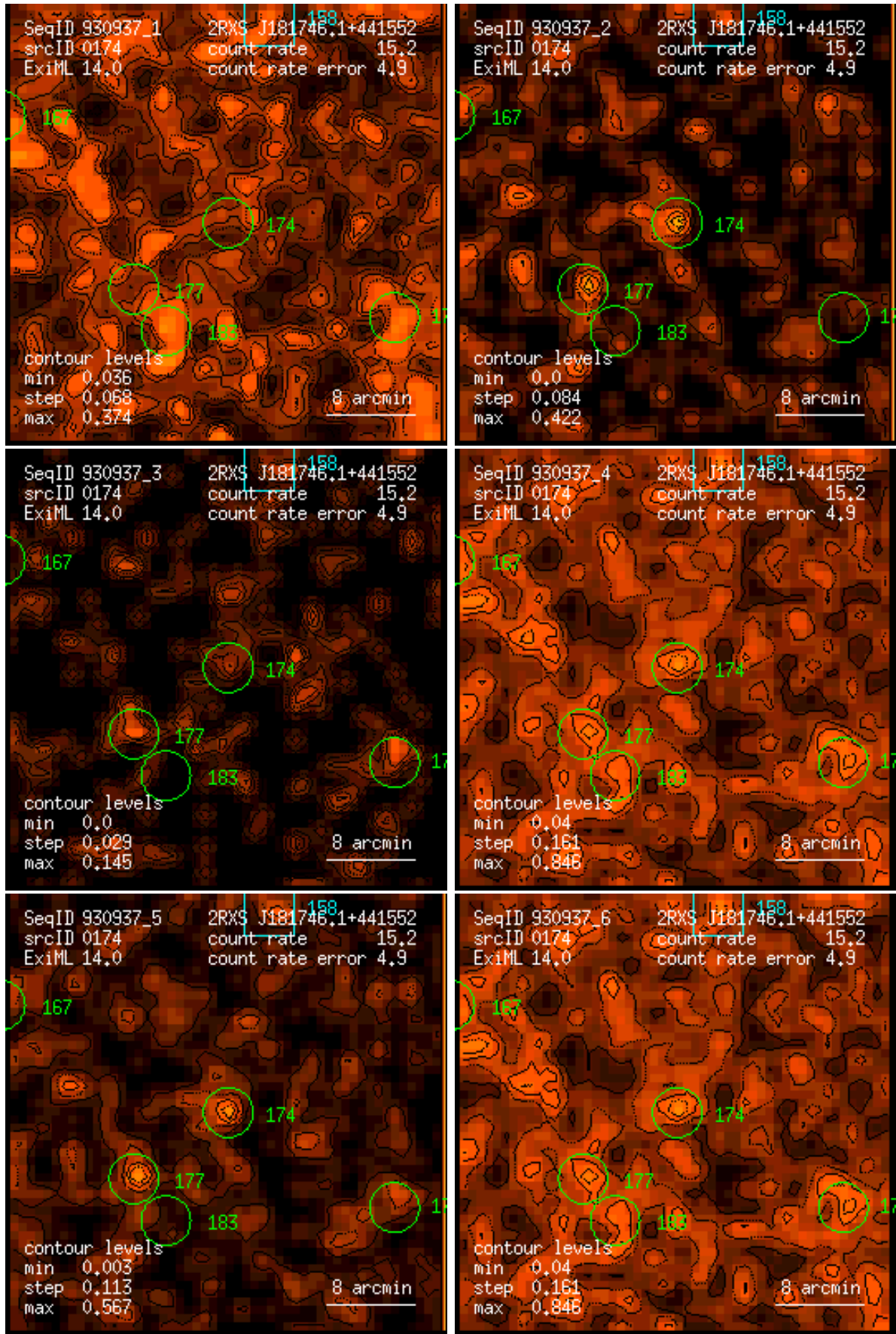
Figure 174: RASS 930937: detection 0174: band rate images, Gaussian filter: (1) PSPC channels 11 – 41, (2) 52 – 90, (3) 91 – 201, (4) 11 – 235, (5) 52 – 201, (6) 11 – 201. Broad band rates in counts/ks. Band rate contour levels in counts/ks/arcmin 2 .
