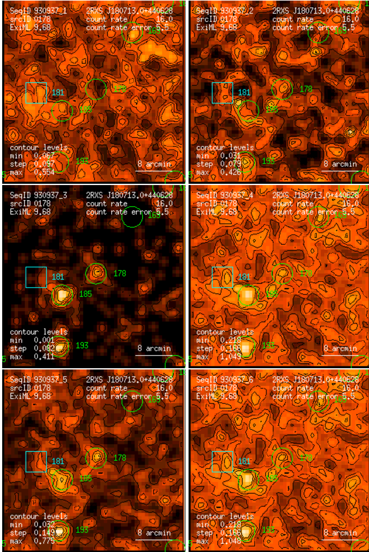
Figure 178: RASS 930937: detection 0178: band rate images, Gaussian filter: (1) PSPC channels 11 – 41, (2) 52 – 90, (3) 91 – 201, (4) 11 – 235, (5) 52 – 201, (6) 11 – 201. Broad band rates in counts/ks. Band rate contour levels in counts/ks/arcmin 2 .
