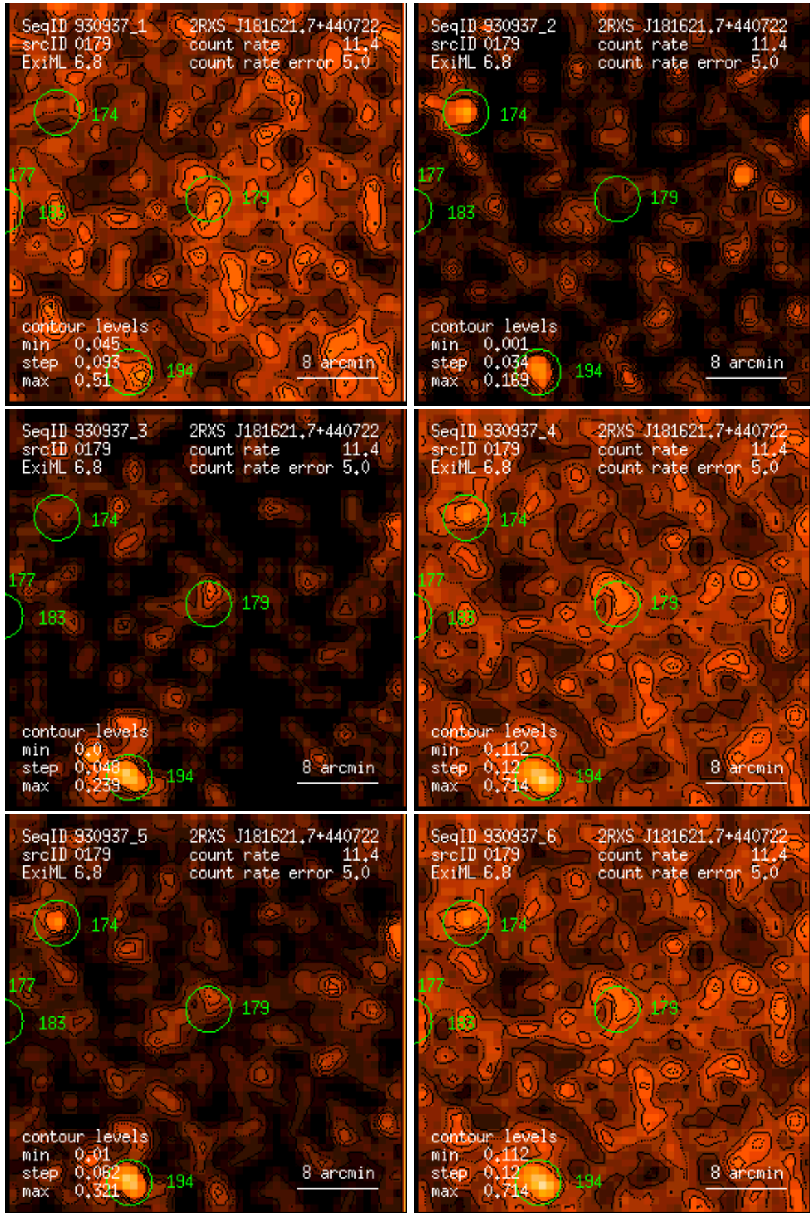
Figure 179: RASS 930937: detection 0179: band rate images, Gaussian filter: (1) PSPC channels 11 – 41, (2) 52 – 90, (3) 91 – 201, (4) 11 – 235, (5) 52 – 201, (6) 11 – 201. Broad band rates in counts/ks. Band rate contour levels in counts/ks/arcmin 2 .
