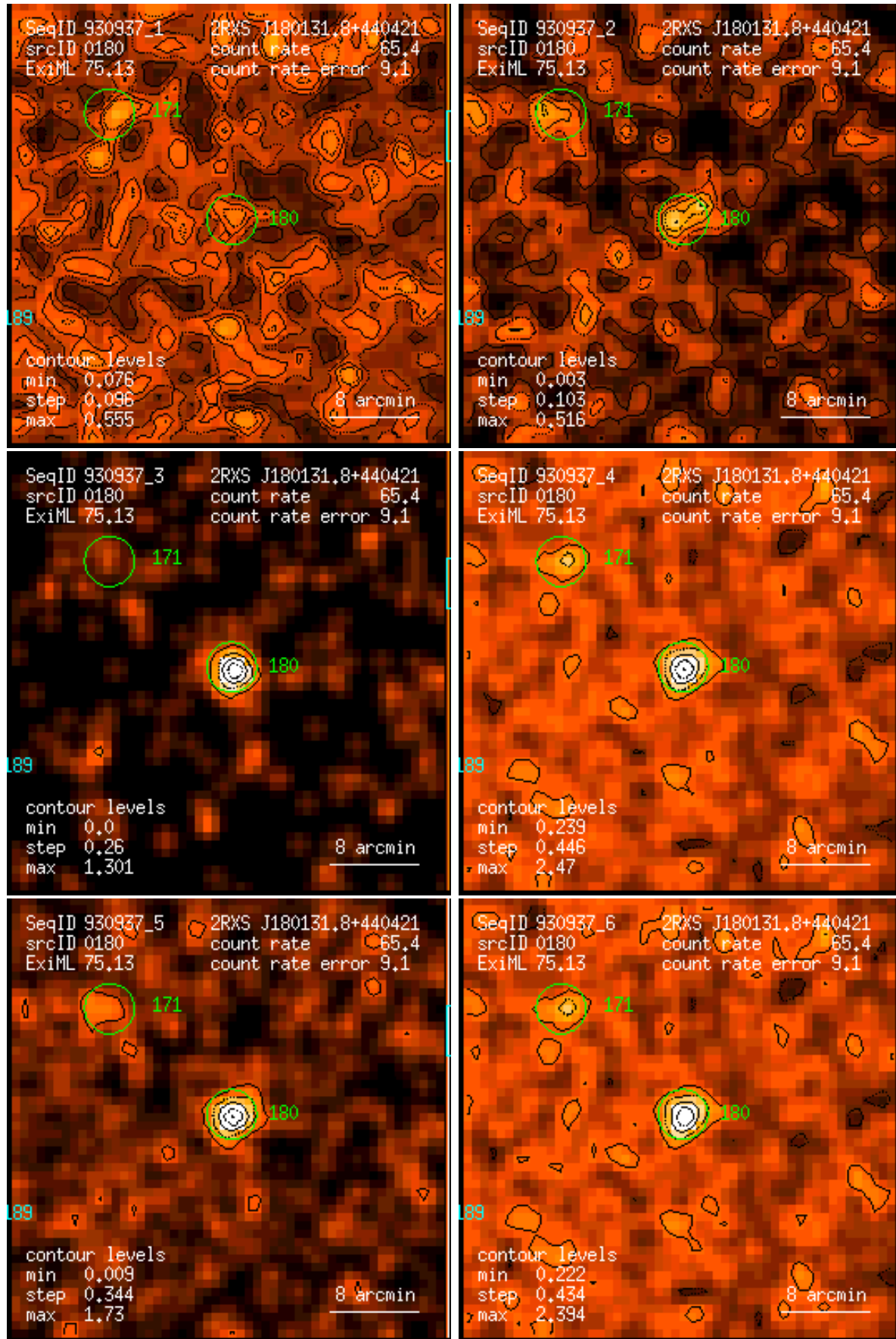
Figure 180: RASS 930937: detection 0180: band rate images, Gaussian filter: (1) PSPC channels 11 – 41, (2) 52 – 90, (3) 91 – 201, (4) 11 – 235, (5) 52 – 201, (6) 11 – 201. Broad band rates in counts/ks. Band rate contour levels in counts/ks/arcmin 2 .
