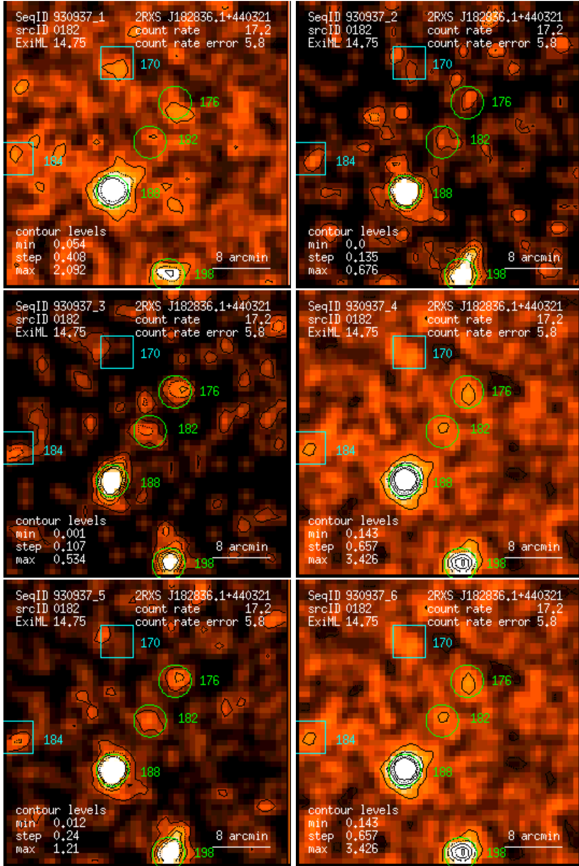
Figure 182: RASS 930937: detection 0182: band rate images, Gaussian filter: (1) PSPC channels 11 – 41, (2) 52 – 90, (3) 91 – 201, (4) 11 – 235, (5) 52 – 201, (6) 11 – 201. Broad band rates in counts/ks. Band rate contour levels in counts/ks/arcmin 2 .
