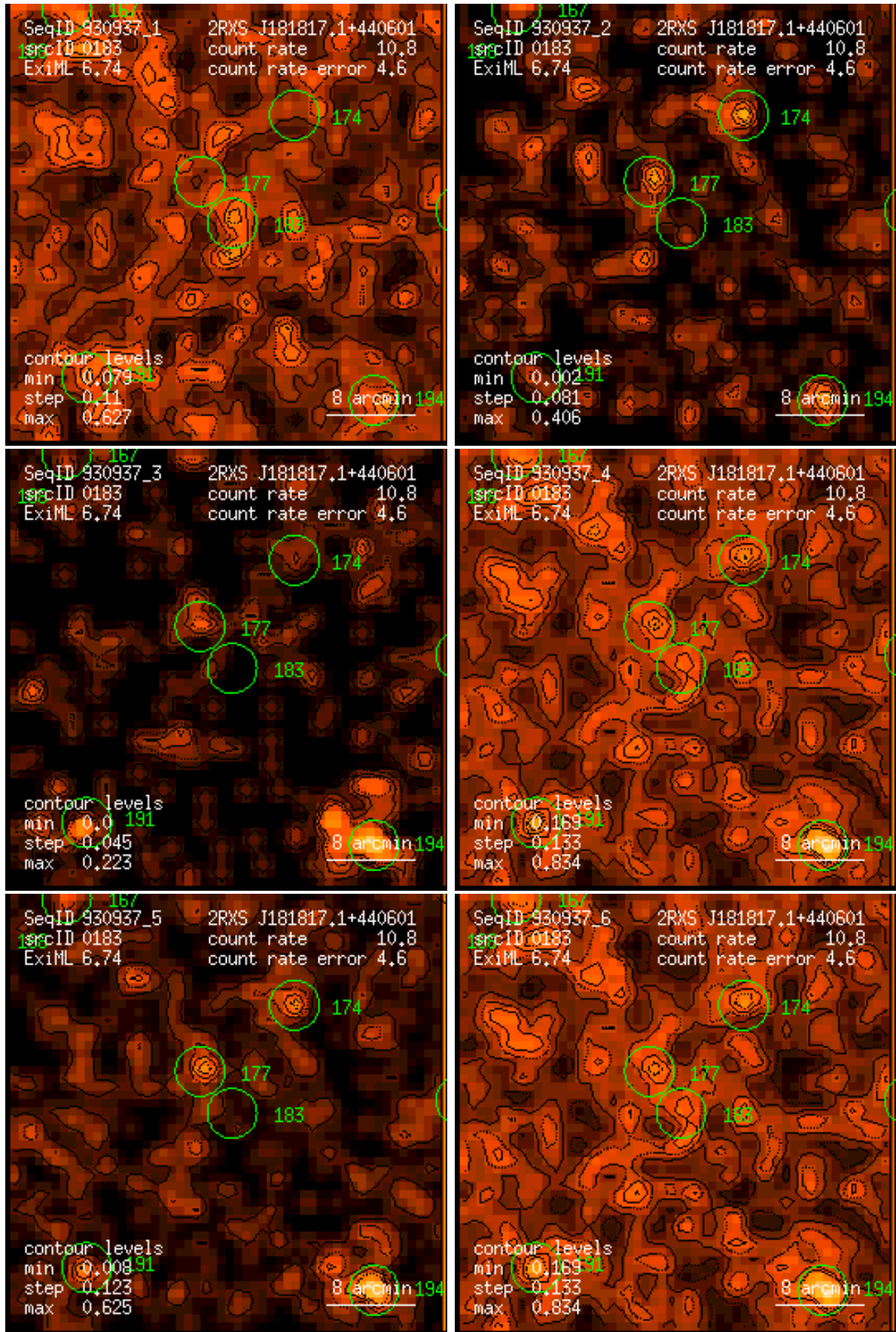
Figure 183: RASS 930937: detection 0183: band rate images, Gaussian filter: (1) PSPC channels 11 – 41, (2) 52 – 90, (3) 91 – 201, (4) 11 – 235, (5) 52 – 201, (6) 11 – 201. Broad band rates in counts/ks. Band rate contour levels in counts/ks/arcmin 2 .
