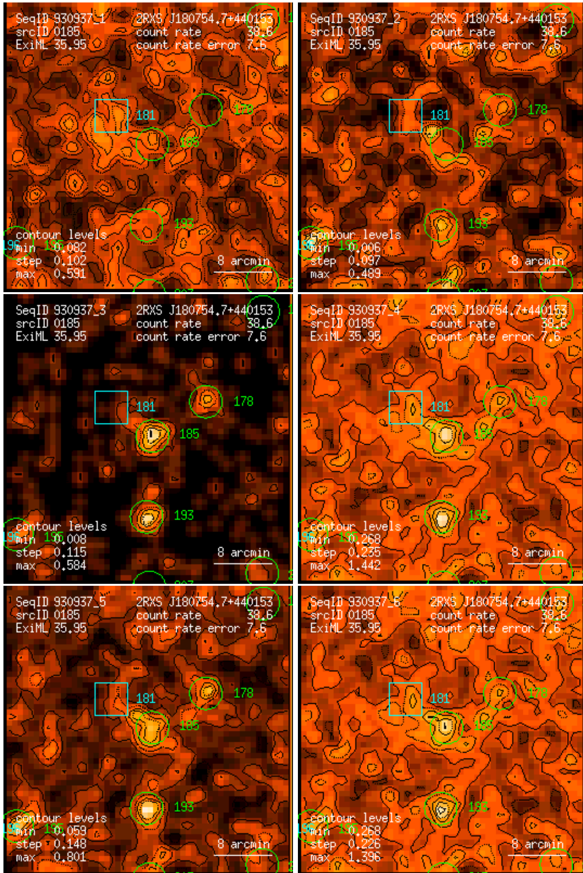
Figure 185: RASS 930937: detection 0185: band rate images, Gaussian filter: (1) PSPC channels 11 – 41, (2) 52 – 90, (3) 91 – 201, (4) 11 – 235, (5) 52 – 201, (6) 11 – 201. Broad band rates in counts/ks. Band rate contour levels in counts/ks/arcmin 2 .
