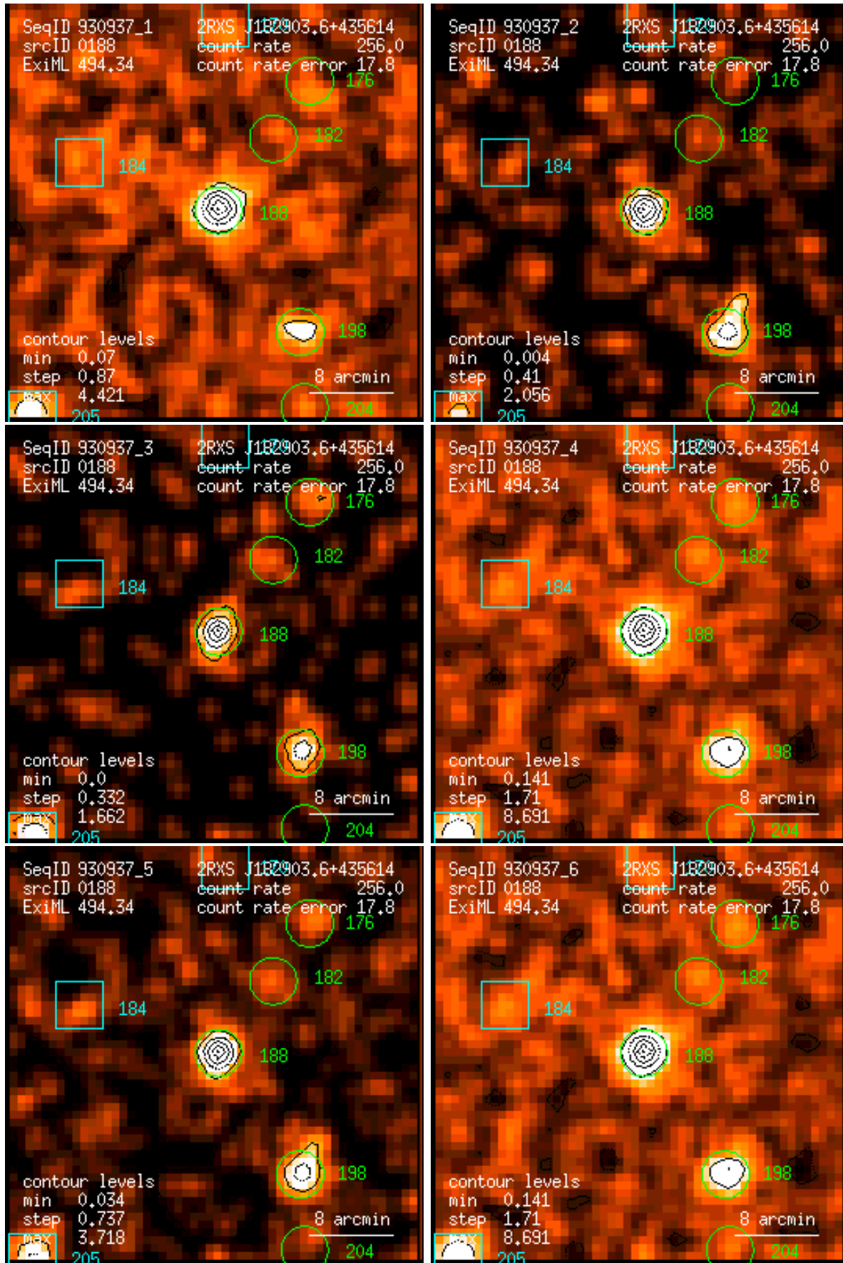
Figure 188: RASS 930937: detection 0188: band rate images, Gaussian filter: (1) PSPC channels 11 – 41, (2) 52 – 90, (3) 91 – 201, (4) 11 – 235, (5) 52 – 201, (6) 11 – 201. Broad band rates in counts/ks. Band rate contour levels in counts/ks/arcmin 2 .
