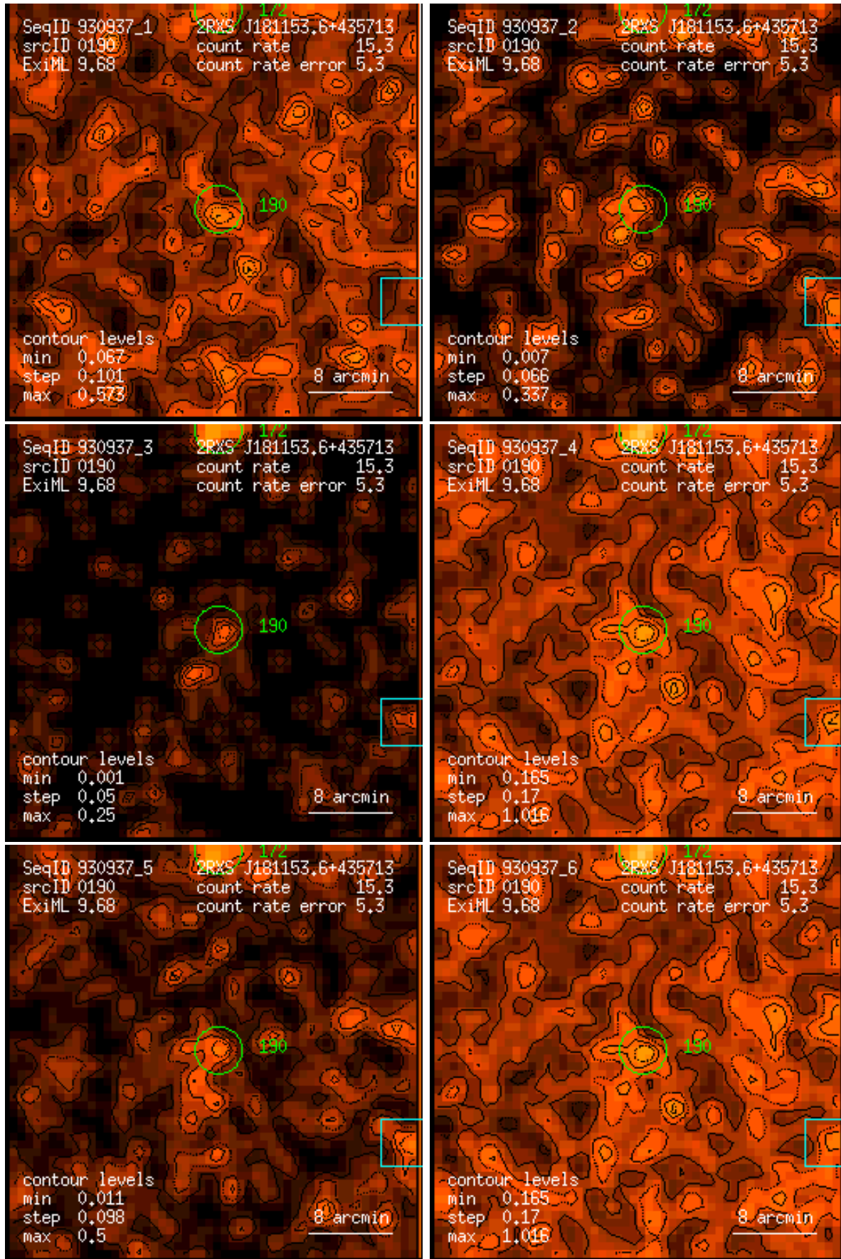
Figure 190: RASS 930937: detection 0190: band rate images, Gaussian filter: (1) PSPC channels 11 – 41, (2) 52 – 90, (3) 91 – 201, (4) 11 – 235, (5) 52 – 201, (6) 11 – 201. Broad band rates in counts/ks. Band rate contour levels in counts/ks/arcmin 2 .
