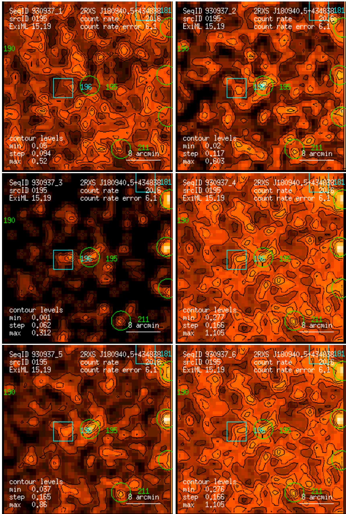
Figure 195: RASS 930937: detection 0195: band rate images, Gaussian filter: (1) PSPC channels 11 – 41, (2) 52 – 90, (3) 91 – 201, (4) 11 – 235, (5) 52 – 201, (6) 11 – 201. Broad band rates in counts/ks. Band rate contour levels in counts/ks/arcmin 2 .
