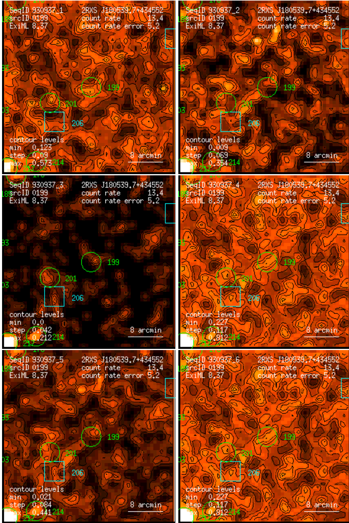
Figure 199: RASS 930937: detection 0199: band rate images, Gaussian filter: (1) PSPC channels 11 – 41, (2) 52 – 90, (3) 91 – 201, (4) 11 – 235, (5) 52 – 201, (6) 11 – 201. Broad band rates in counts/ks. Band rate contour levels in counts/ks/arcmin 2 .
