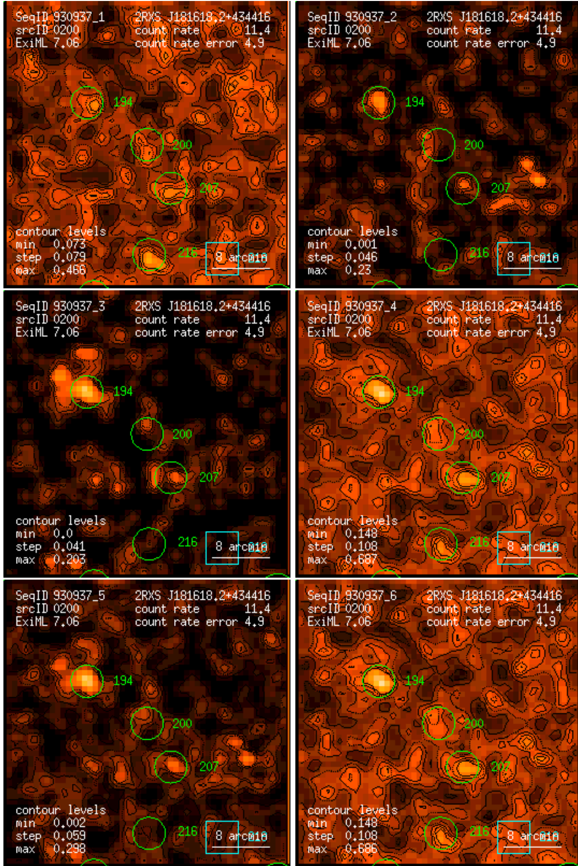
Figure 200: RASS 930937: detection 0200: band rate images, Gaussian filter: (1) PSPC channels 11 – 41, (2) 52 – 90, (3) 91 – 201, (4) 11 – 235, (5) 52 – 201, (6) 11 – 201. Broad band rates in counts/ks. Band rate contour levels in counts/ks/arcmin 2 .
