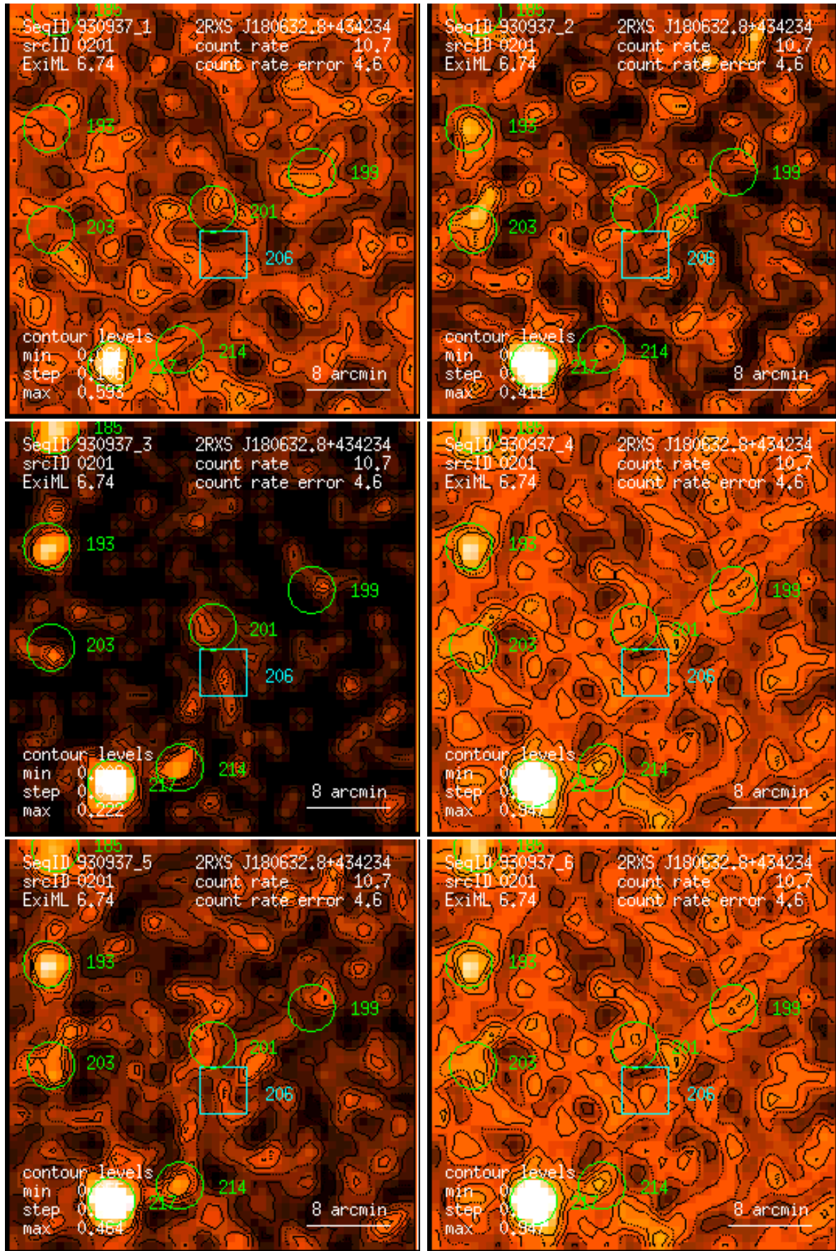
Figure 201: RASS 930937: detection 0201: band rate images, Gaussian filter: (1) PSPC channels 11 – 41, (2) 52 – 90, (3) 91 – 201, (4) 11 – 235, (5) 52 – 201, (6) 11 – 201. Broad band rates in counts/ks. Band rate contour levels in counts/ks/arcmin 2 .
