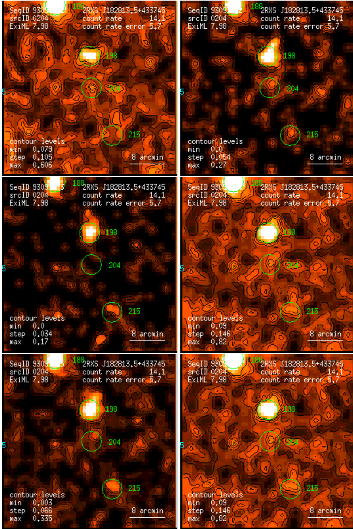
Figure 204: RASS 930937: detection 0204: band rate images, Gaussian filter: (1) PSPC channels 11 – 41, (2) 52 – 90, (3) 91 – 201, (4) 11 – 235, (5) 52 – 201, (6) 11 – 201. Broad band rates in counts/ks. Band rate contour levels in counts/ks/arcmin 2 .
