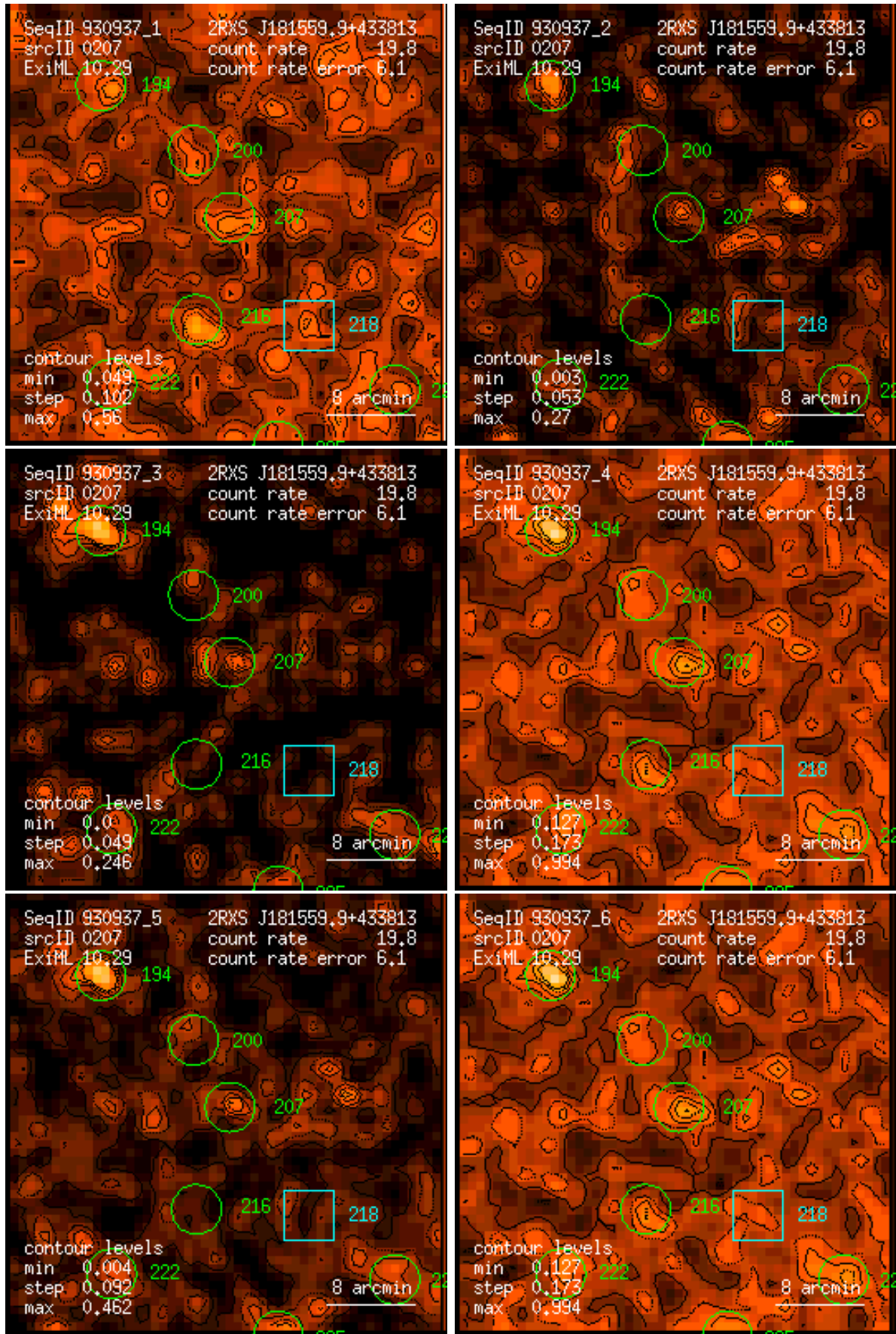
Figure 207: RASS 930937: detection 0207: band rate images, Gaussian filter: (1) PSPC channels 11 – 41, (2) 52 – 90, (3) 91 – 201, (4) 11 – 235, (5) 52 – 201, (6) 11 – 201. Broad band rates in counts/ks. Band rate contour levels in counts/ks/arcmin 2 .
