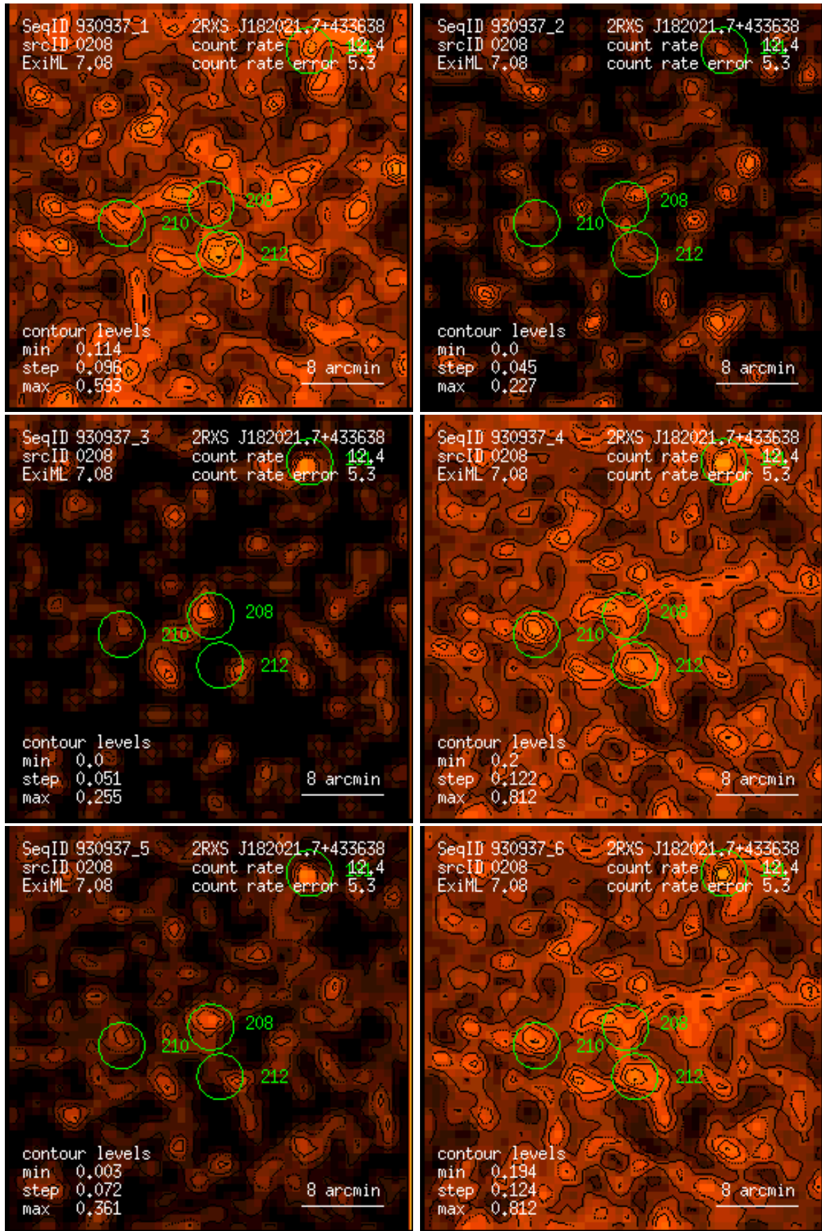
Figure 208: RASS 930937: detection 0208: band rate images, Gaussian filter: (1) PSPC channels 11 – 41, (2) 52 – 90, (3) 91 – 201, (4) 11 – 235, (5) 52 – 201, (6) 11 – 201. Broad band rates in counts/ks. Band rate contour levels in counts/ks/arcmin 2 .
