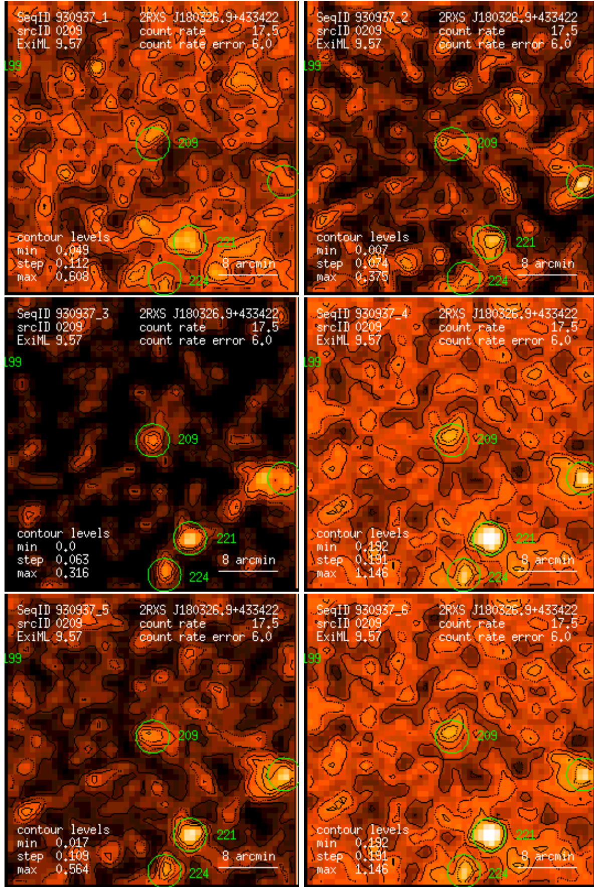
Figure 209: RASS 930937: detection 0209: band rate images, Gaussian filter: (1) PSPC channels 11 – 41, (2) 52 – 90, (3) 91 – 201, (4) 11 – 235, (5) 52 – 201, (6) 11 – 201. Broad band rates in counts/ks. Band rate contour levels in counts/ks/arcmin 2 .
