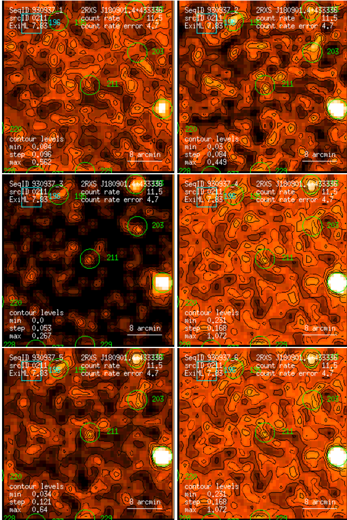
Figure 211: RASS 930937: detection 0211: band rate images, Gaussian filter: (1) PSPC channels 11 – 41, (2) 52 – 90, (3) 91 – 201, (4) 11 – 235, (5) 52 – 201, (6) 11 – 201. Broad band rates in counts/ks. Band rate contour levels in counts/ks/arcmin 2 .
