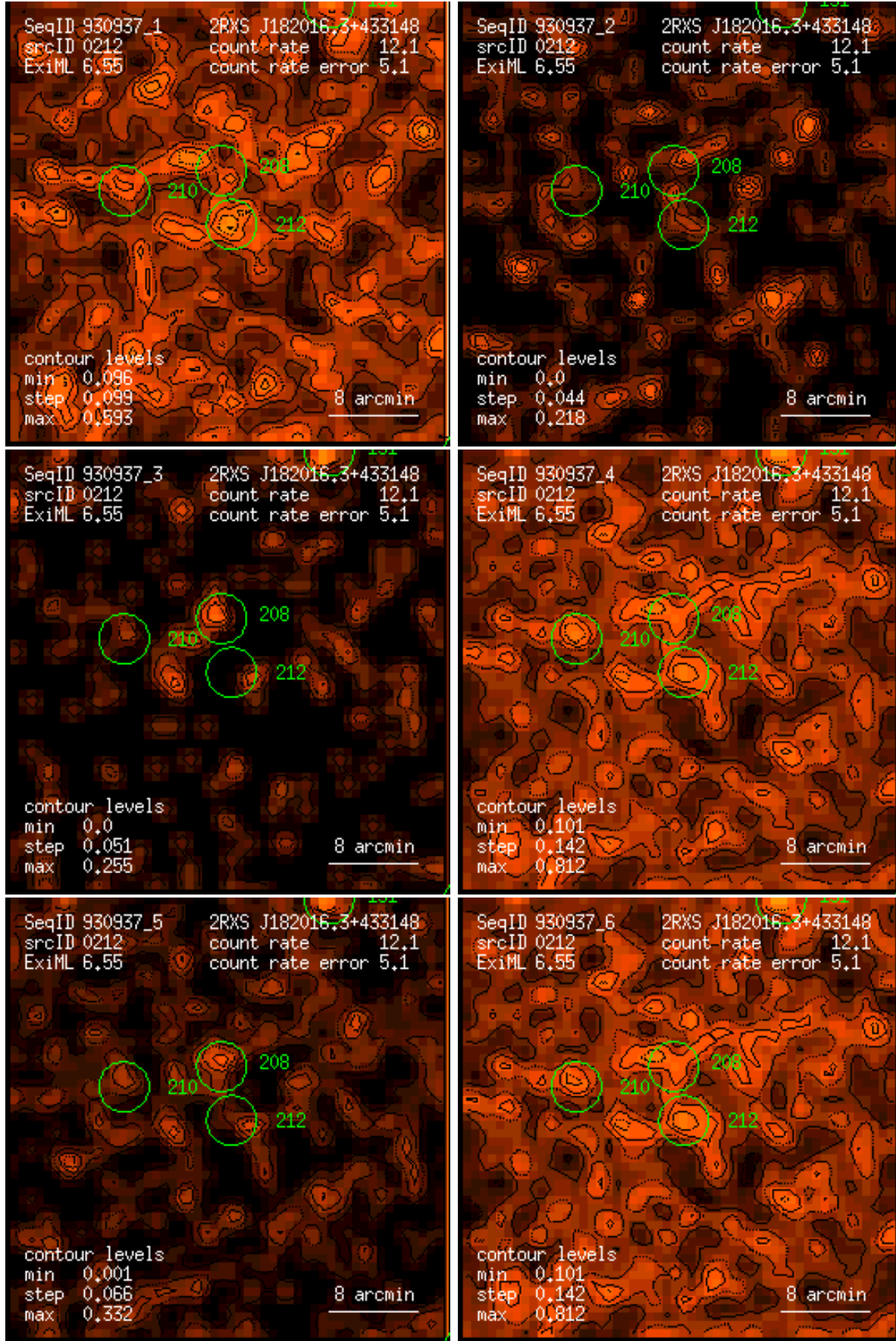
Figure 212: RASS 930937: detection 0212: band rate images, Gaussian filter: (1) PSPC channels 11 – 41, (2) 52 – 90, (3) 91 – 201, (4) 11 – 235, (5) 52 – 201, (6) 11 – 201. Broad band rates in counts/ks. Band rate contour levels in counts/ks/arcmin 2 .
